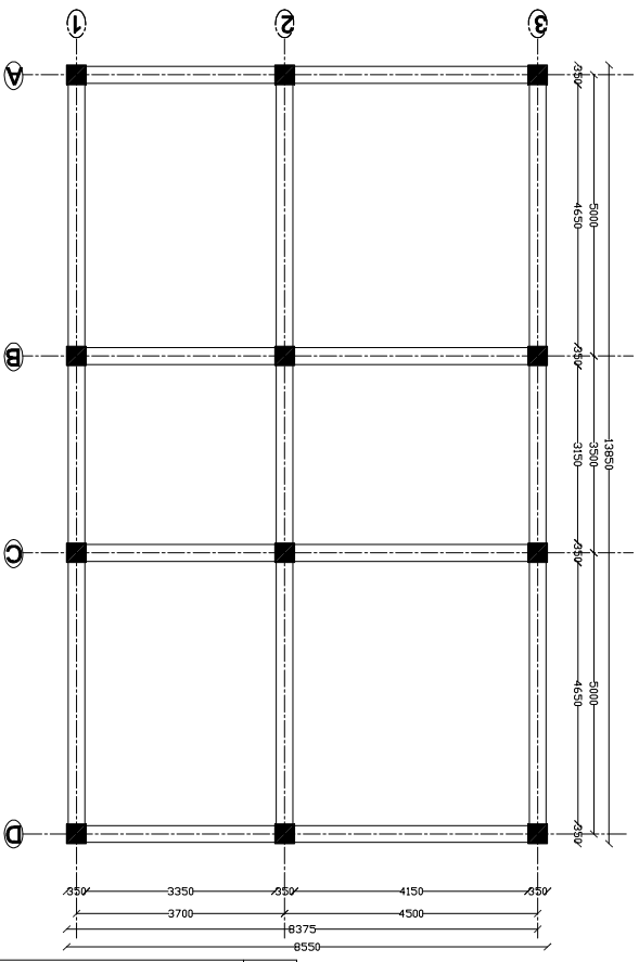
FLOOR BEAM LAYOUT PLAN [clear-section350*300mm]
