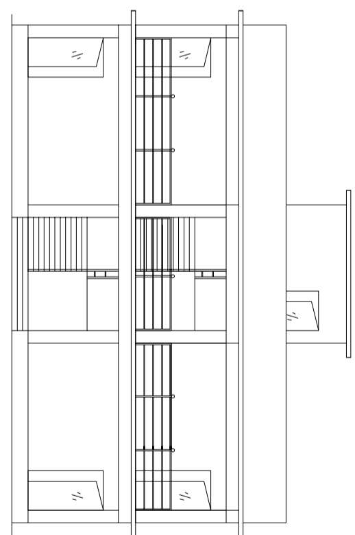
NORTH ELEVATION
