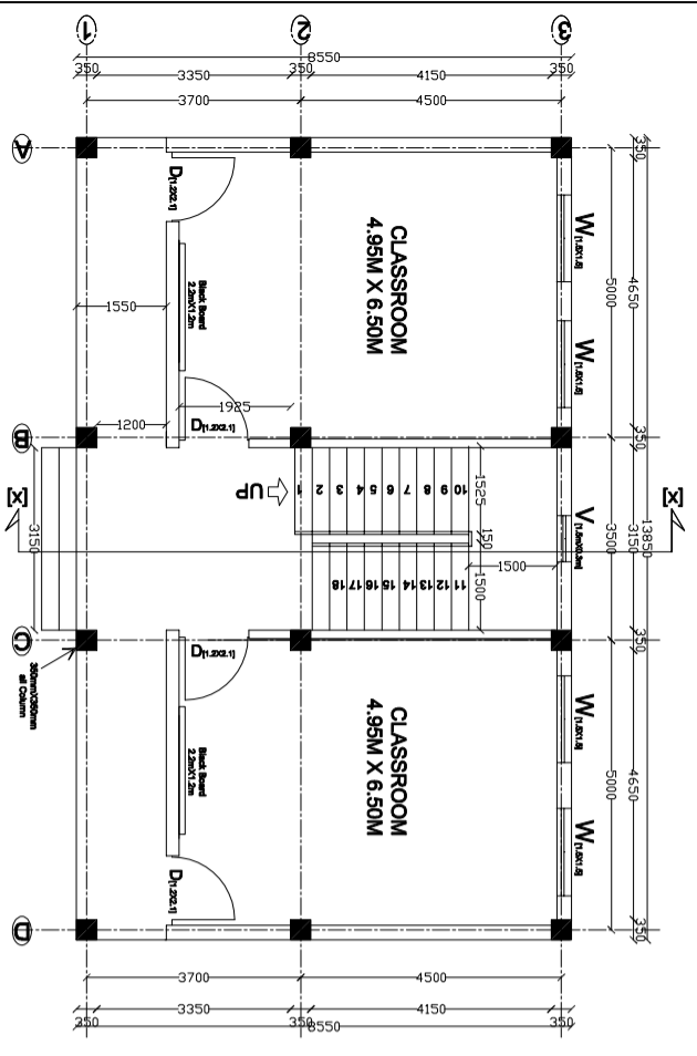
GROUND FLOOR PLAN PLINTH AREA : 118.42sq.m
