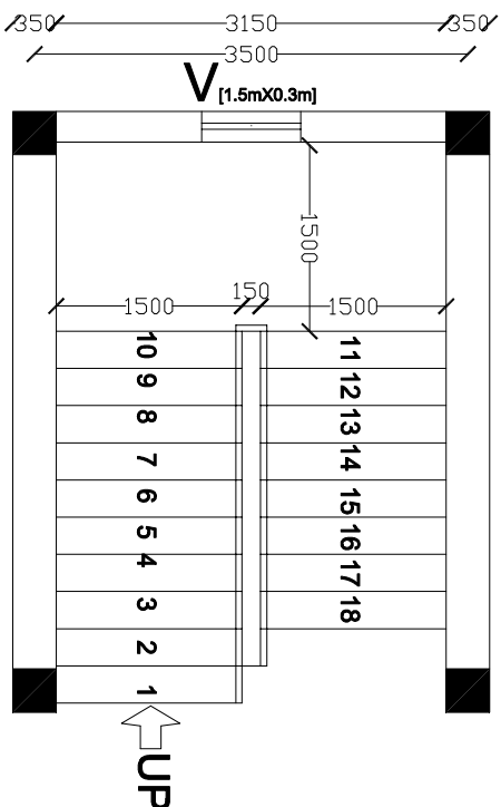
STAIRCASE PLAN
