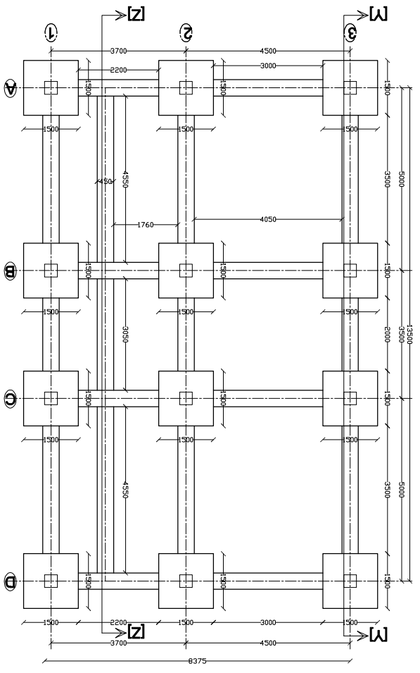
TRENCH PLAN
