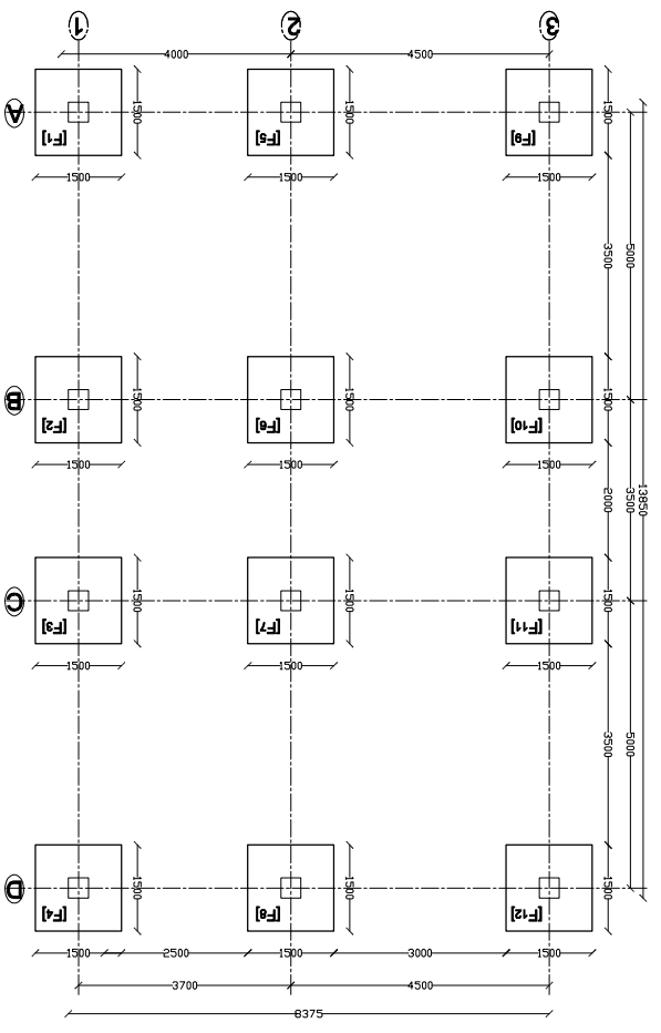
FOOTING PLAN
