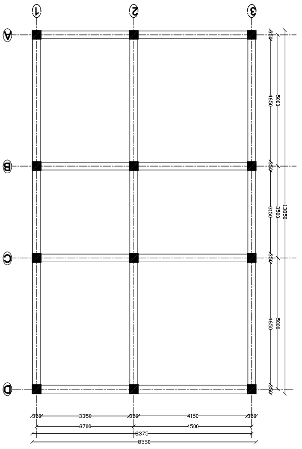
PLINTH BEAM LAYOUT PLAN [350*300mm]
