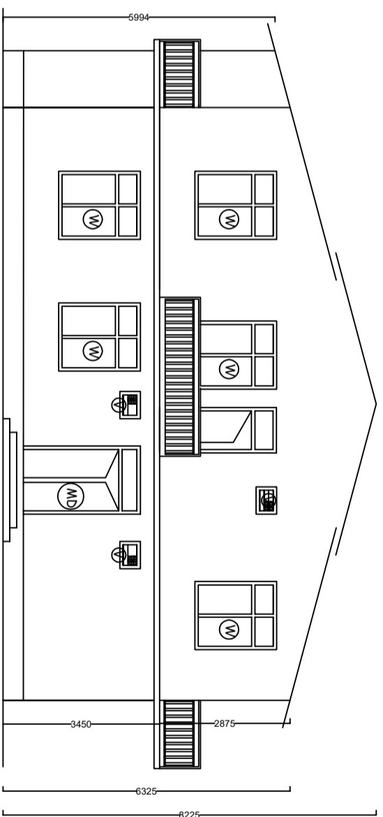
NORTH ELEVATION (BACK)
