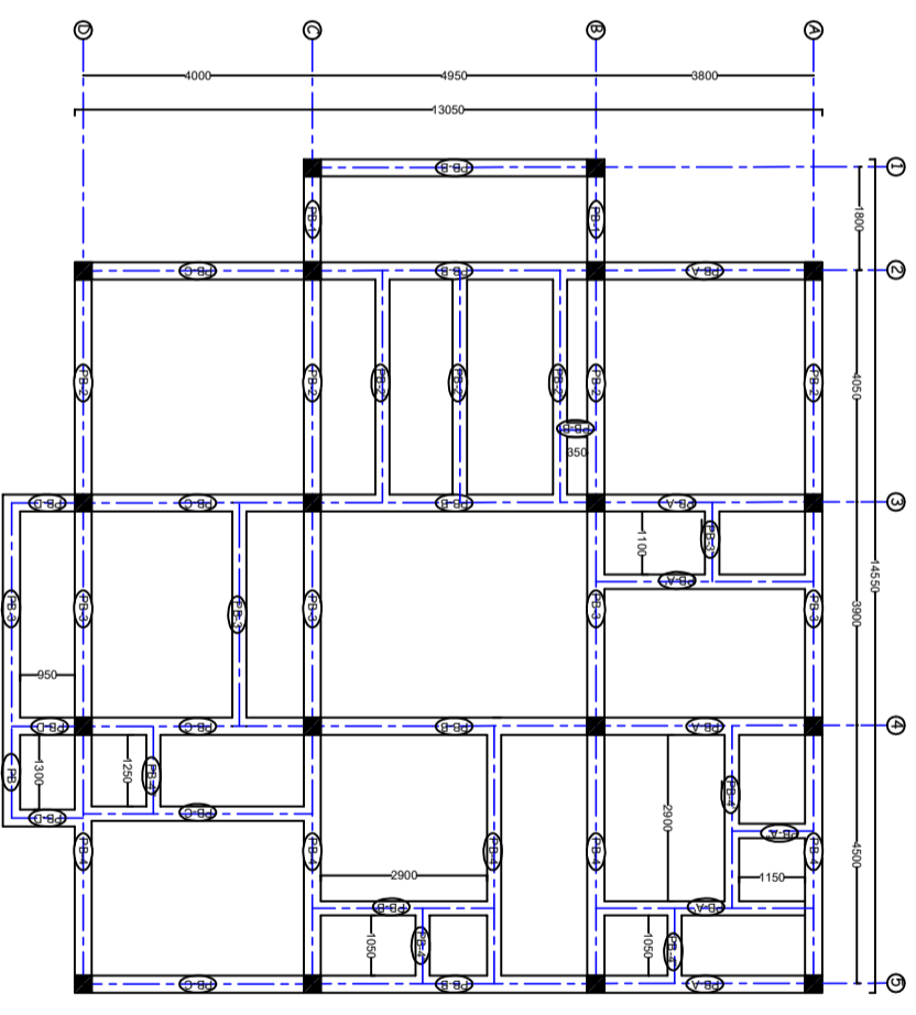
PLINTH BEAM PLAN
