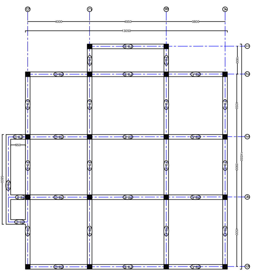
FLOOR BEAM PLAN
