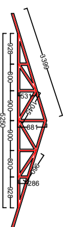
CENTER TRUSS
