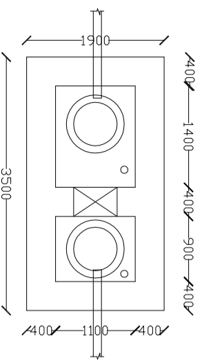
PLAN septic tank 2.3mx1.1m [20users for 2 years]
