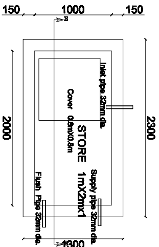
DISTRIBUTION TANK PLAN
