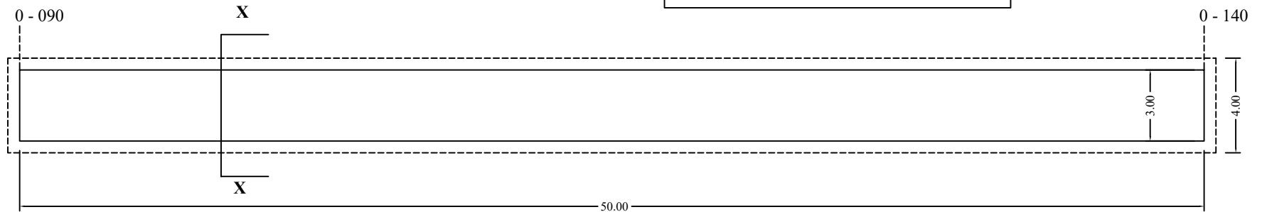
Plan of Gabion Wall (Ch 0-090 to 0-140 m)
