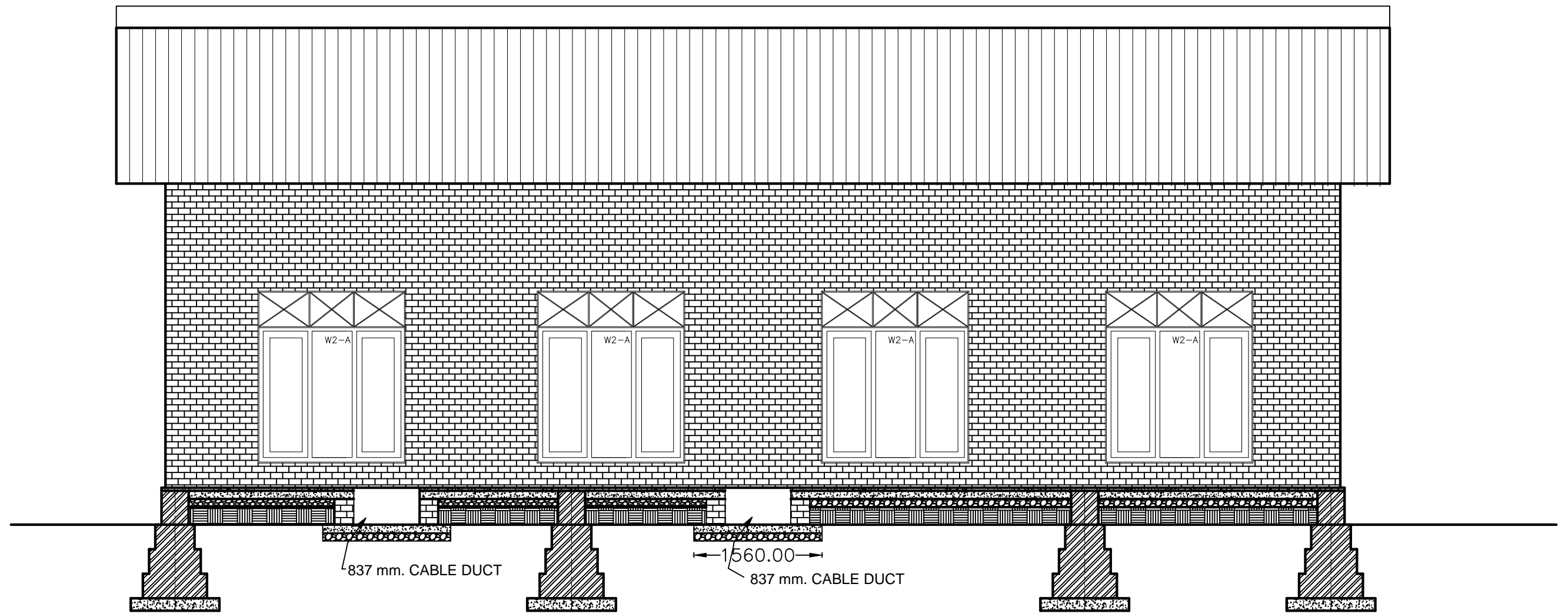
REAR VIEW OF CONTROL ROOM BUILDING (14.5 X 9.00 M)
