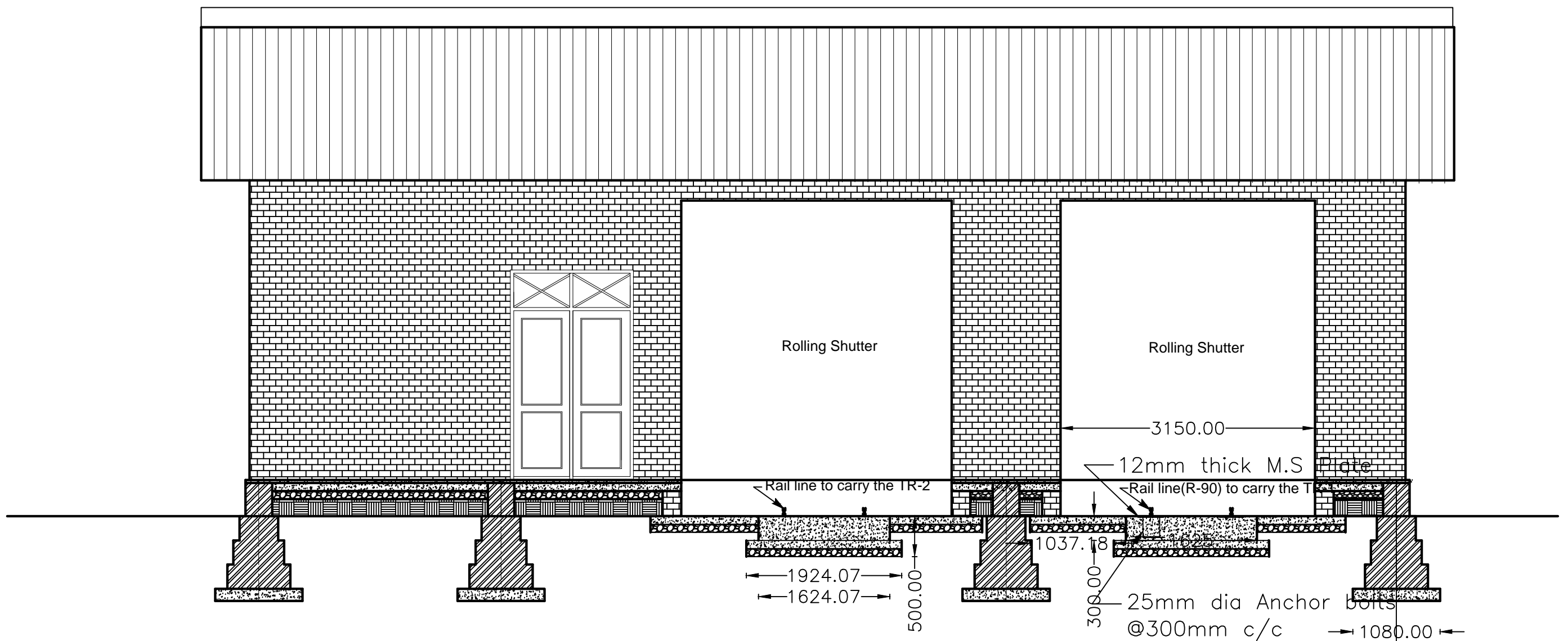
FRONT VIEW OF CONTROL ROOM BUILDING (14.5 X 9.00 M)
