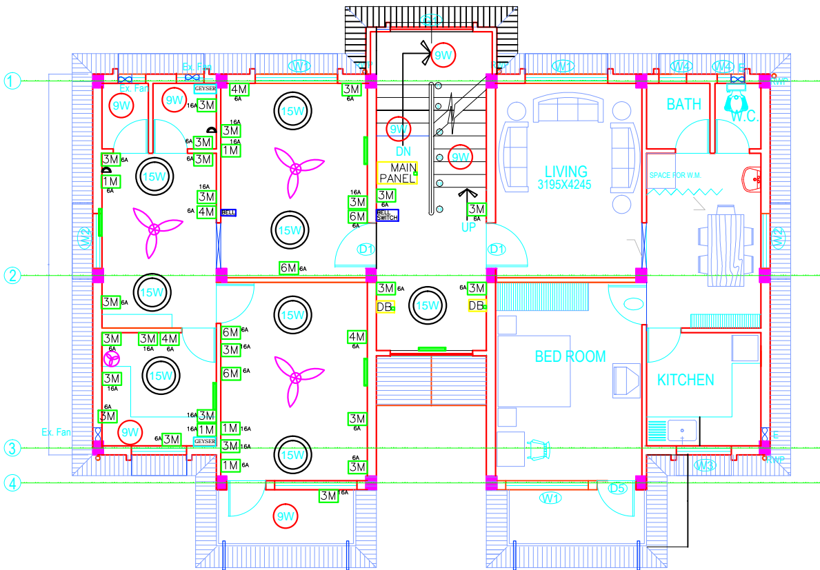
TYPICAL ELECTRICAL INSTALLATION DRAWING POWER HOUSE COLONY_FAMILY ACCOMODATION
