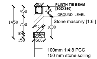
WALL SECTION AT M-M
