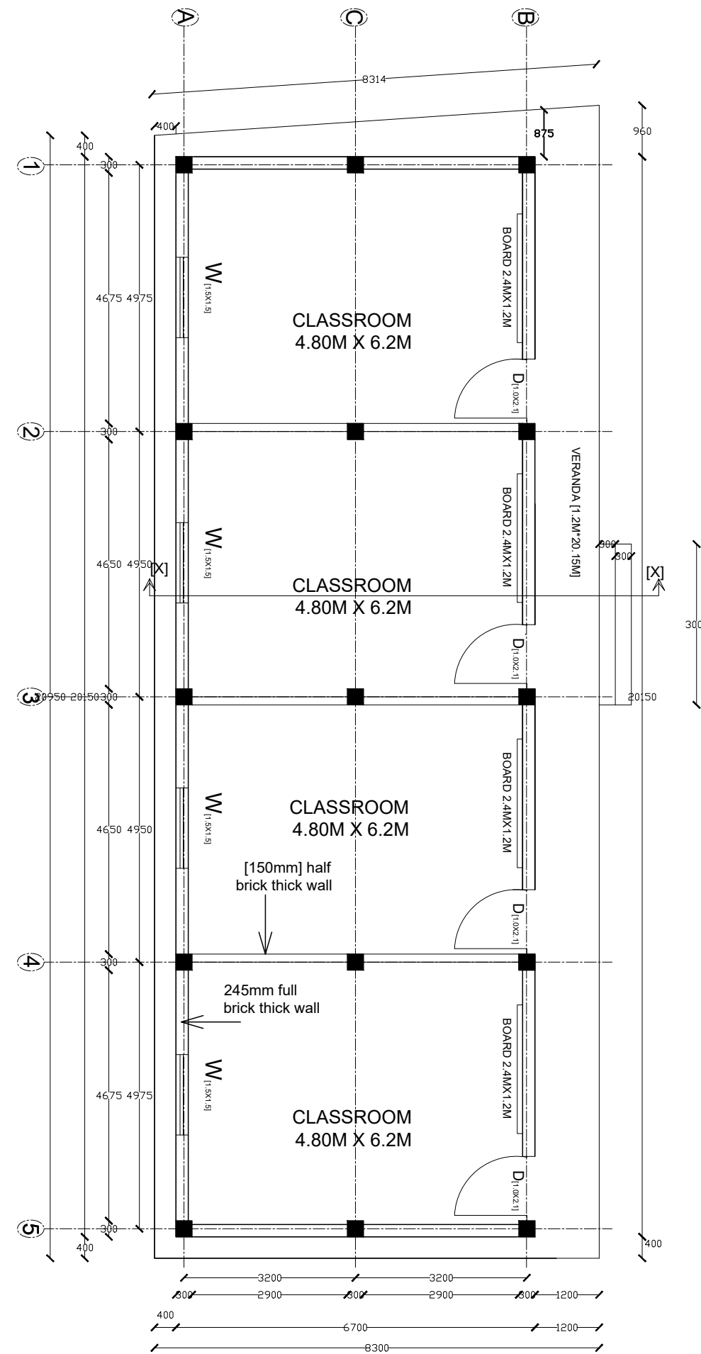
PR.GROUND FLOOR PLAN PLINTH AREA : 135.00sq.m
