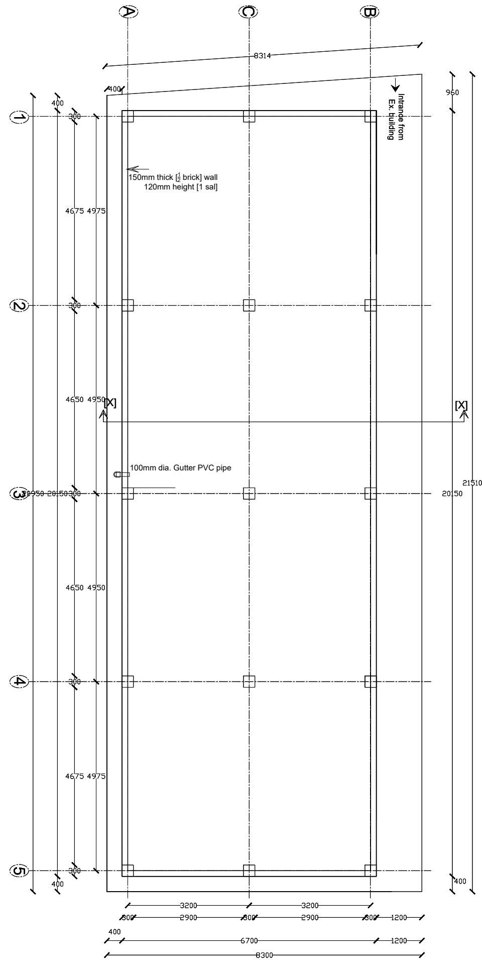
PR ROOF PLAN COVER AREA : 169.88sq.m
