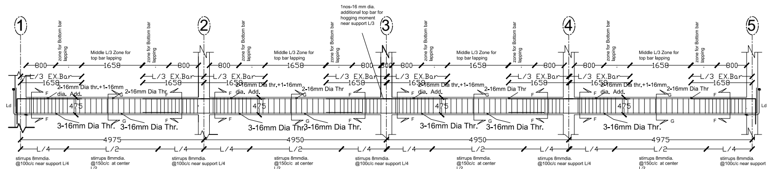
FIRST FLOOR BEAM L-Section along A-A & B-B
