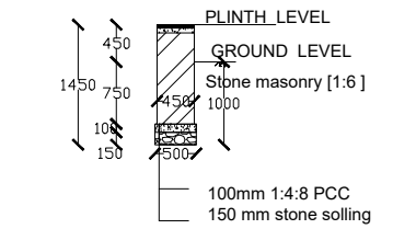
WALL SECTION AT N-N [D-D GRID]
