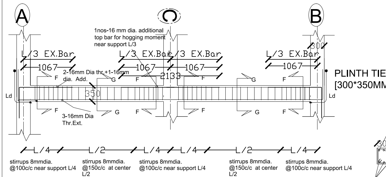
FIRST FLOOR BEAM L-Section along 1-1,...5-5
