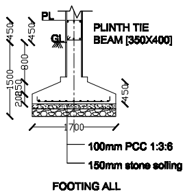
FOOTING ALL
