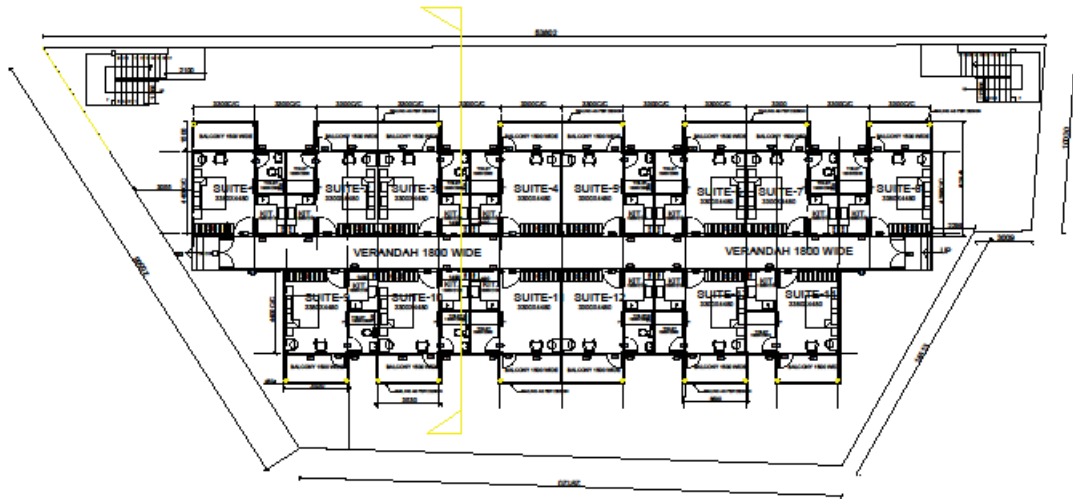
GROUND FLOOR PLAN B4
