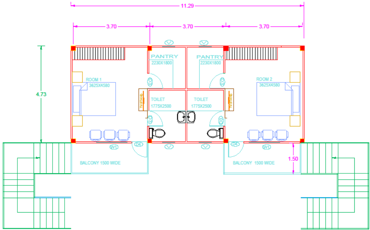
DISPENSARY BUILDING FIRST FLOOR
