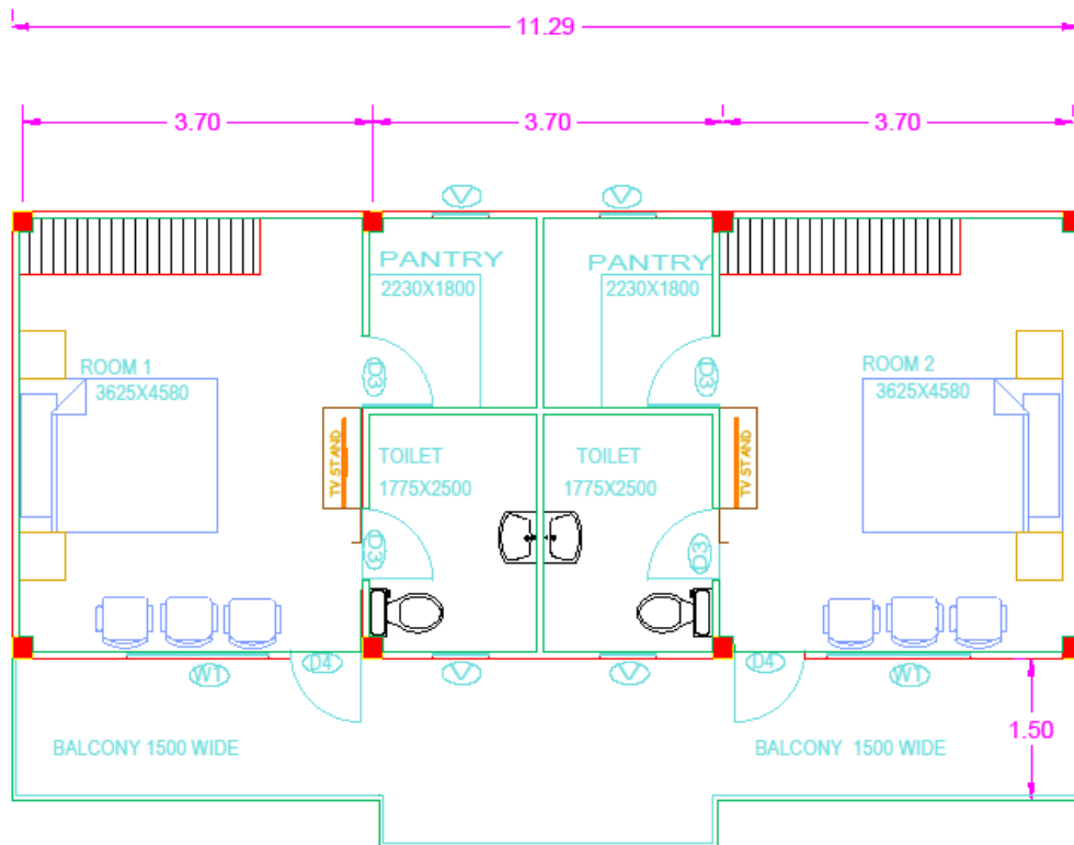
DISPENSARY BUILDING GROUND FLOOR
