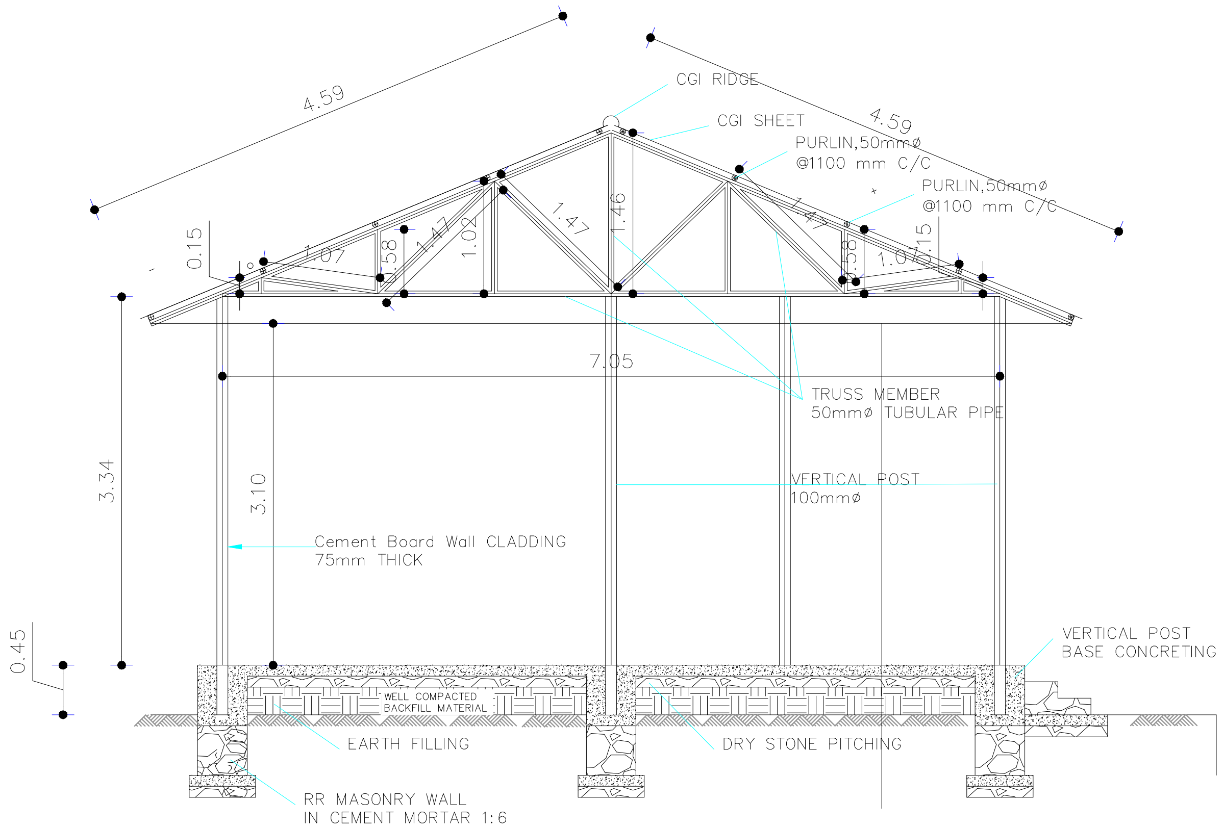
X-SECTION B-B''
