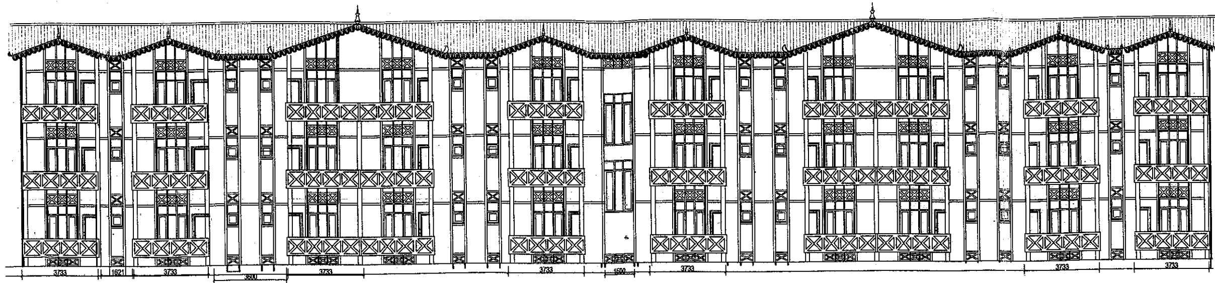
VALLEY SIDE ELEVATION
