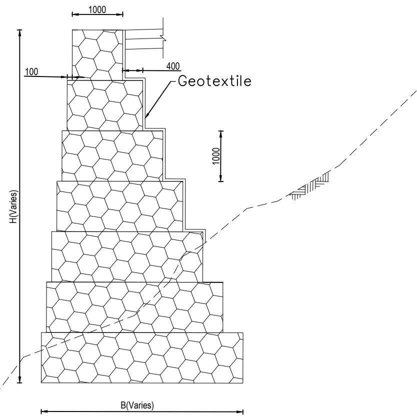
Typical Section of Masonry Breast wall Scale 1:30
