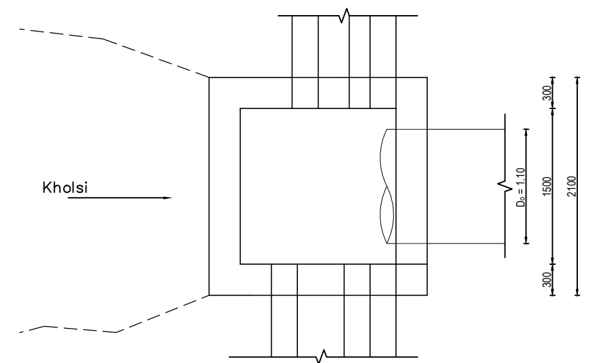
Plan of Catchpit for 900mm HP Scale 1:50
