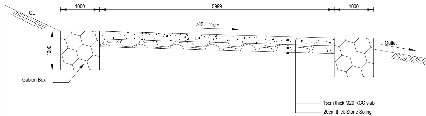
Section at A-A Scale 1:50
