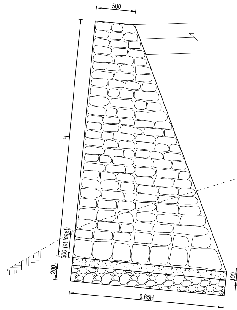
Typical Section of Masonry Retaining Wall Scale 1:30
