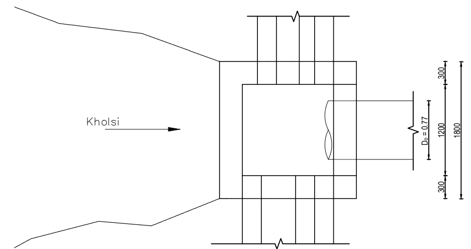
Plan of Catchpit for 600mm HP Scale 1:50
