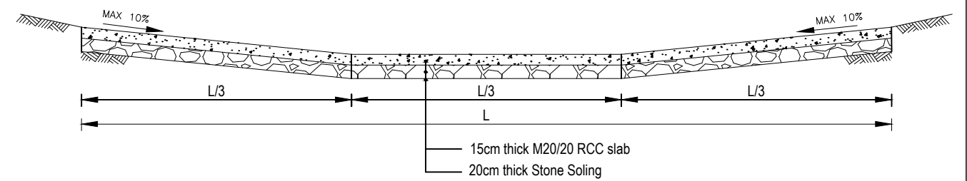
Section at B-B Scale 1:100
