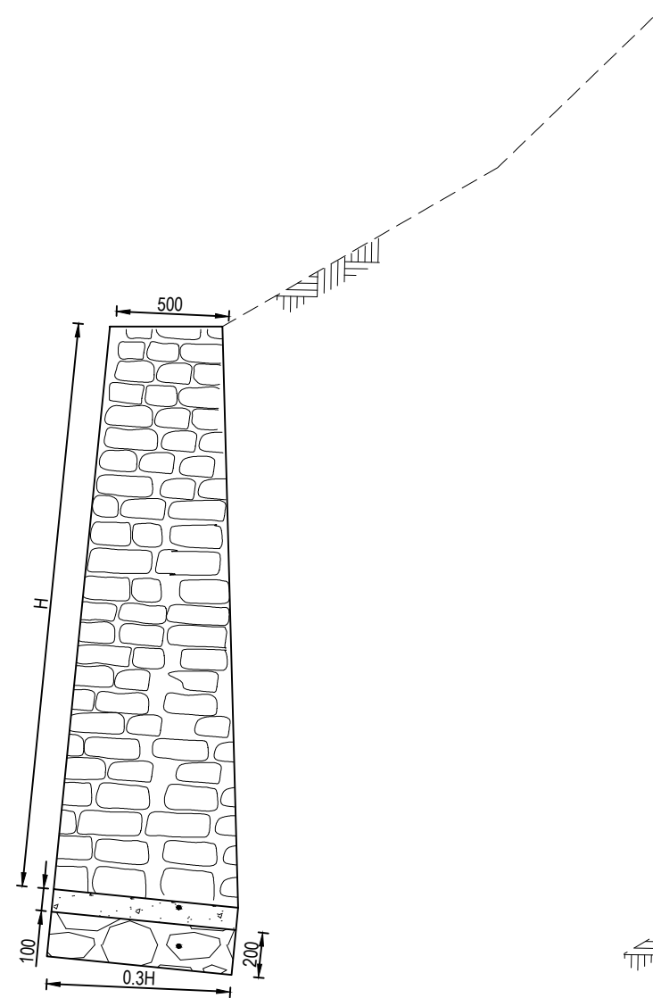
Typical Section of Masonry Breast wall Scale 1:30
