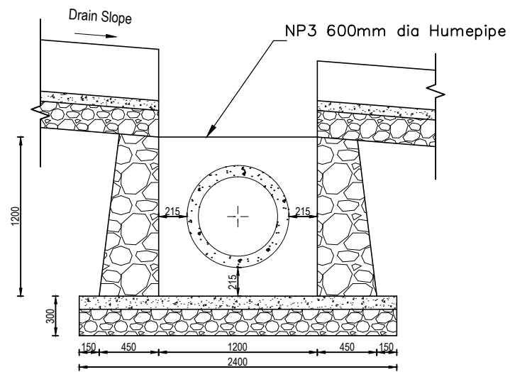
Typical section of Catchpit for 600mm HP Scale 1:40
