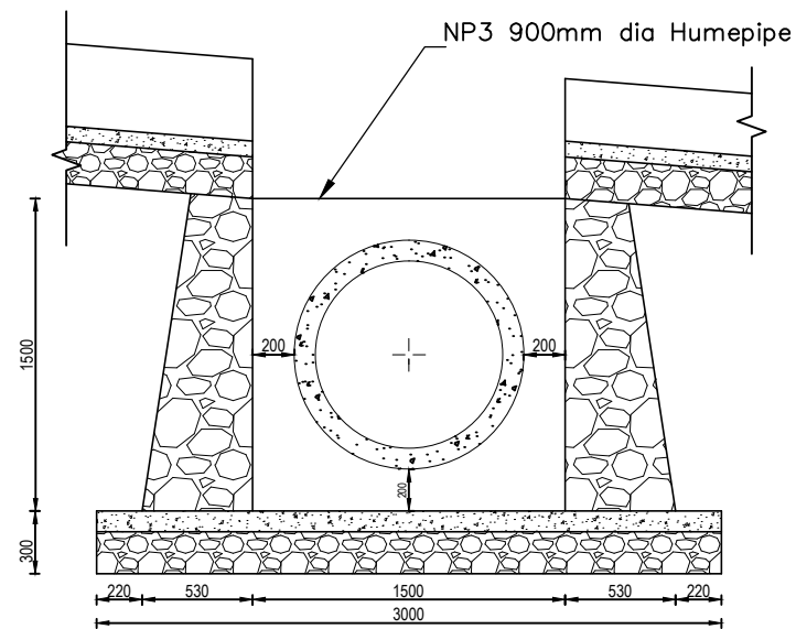
Typical section of Catchpit for 900mm HP Scale 1:40
