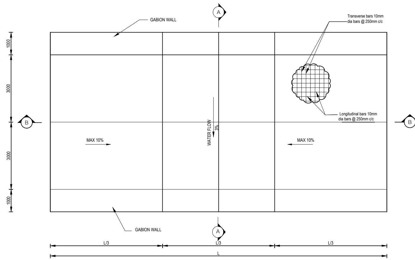
Causeway Plan Scale 1:75
