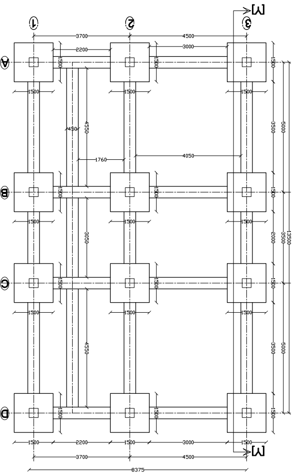
TRENCH PLAN
