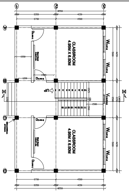
GROUND FLOOR PLAN PLINTH AREA : 118.42sq.m
