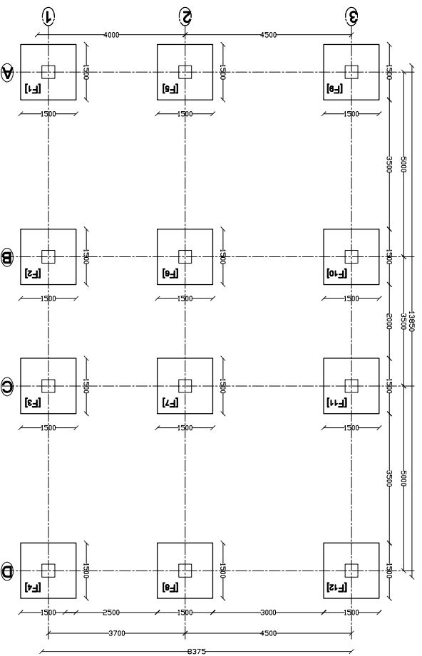
FOOTING PLAN
