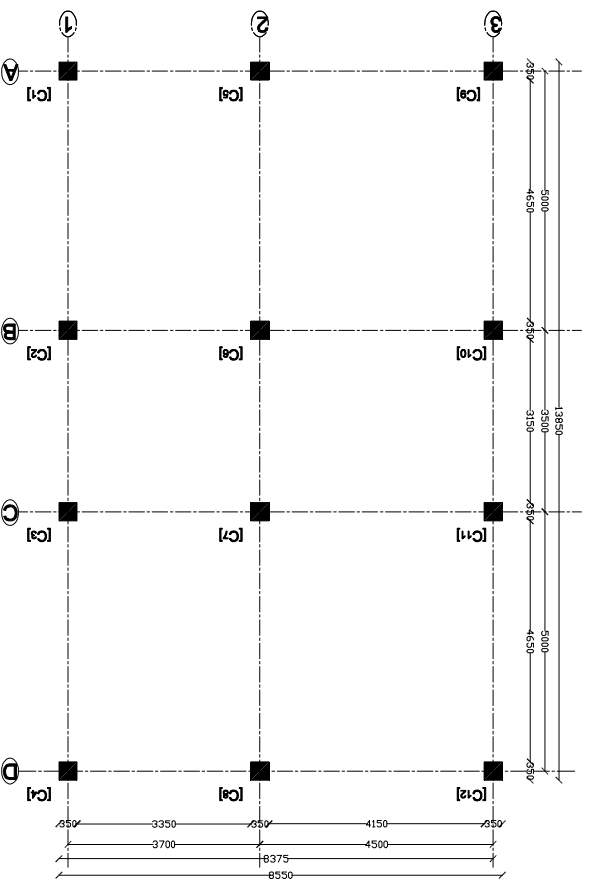
COLUMN PLAN size of column 350mmX350mm
