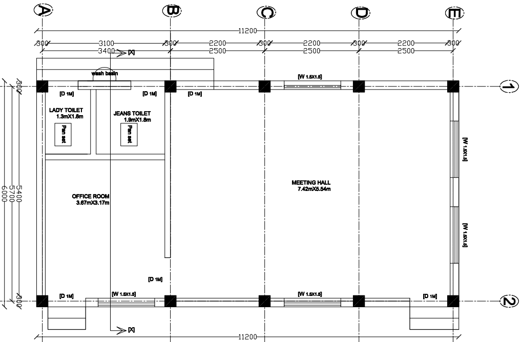
GROUND FLOOR PLAN Plinth Area:67.2sq.m
