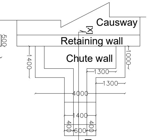
Retaining wall 2 mtr Hight
