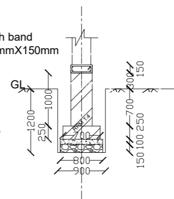
Wall section and stone footing Details
