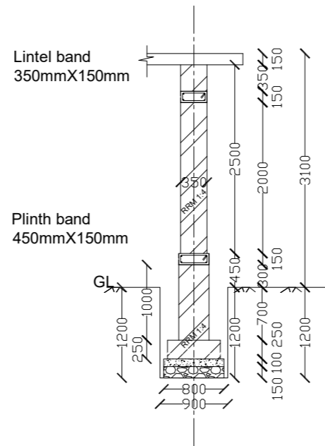
Wall section and stone footing Details
