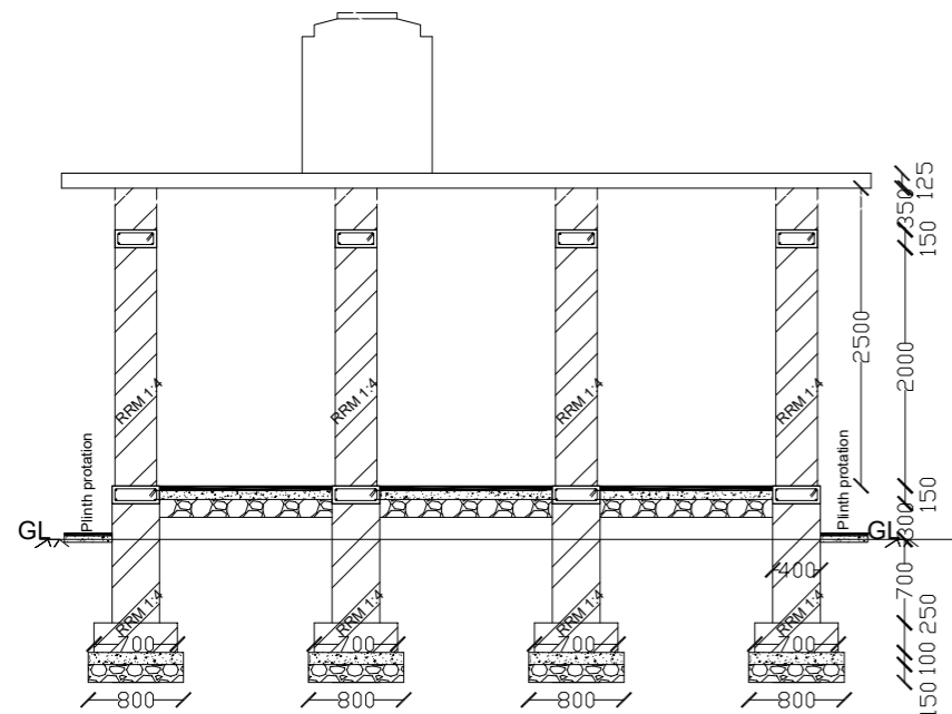
Toilet Section at X-X
