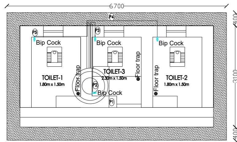
Plinth proction
