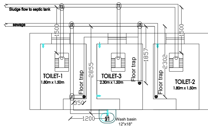
SEWAGE PIPE LAYOUT PLAN
