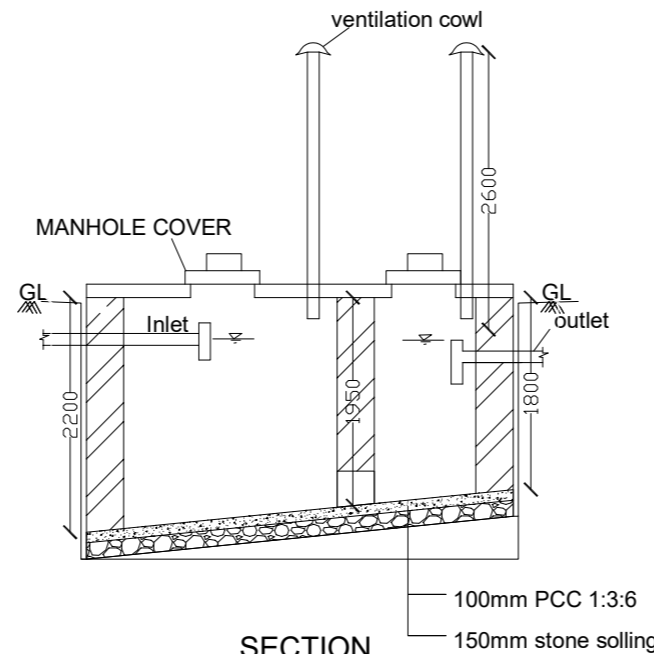
SECTION SEPTIC TANK
