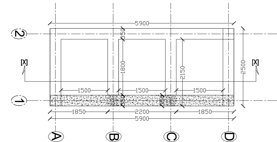
RRM wall super structure Lintel [350mmX150mm]
