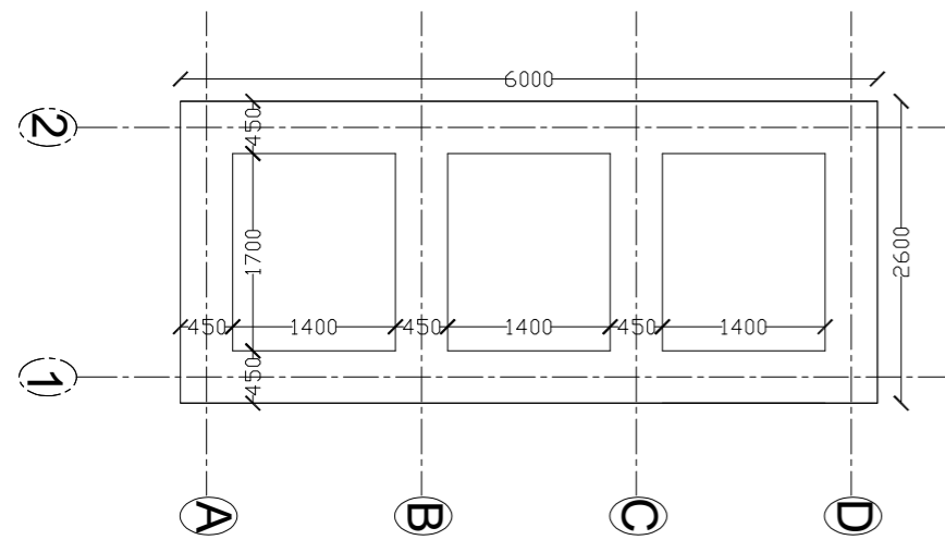
RRM below plinth & Plinth band [450mmX150mm] Plan
