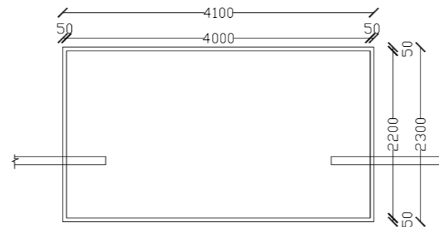
FOUNDATION EXCAVATION PLAN SEPTIC TANK
