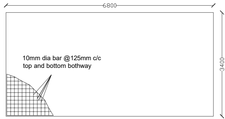
RCC Slab Plan
