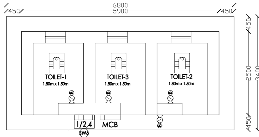
ELECTRICAL WORK LAYOUT
