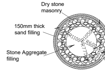
PLAN SOAK PIT
