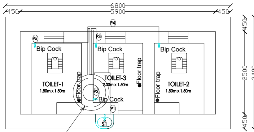
WATER SUPPLY LAYOUT
