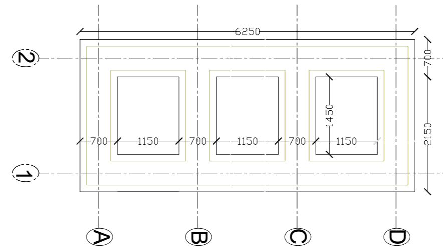
RRM 1st Footing Plan
