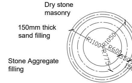
PLAN SOAK PIT
