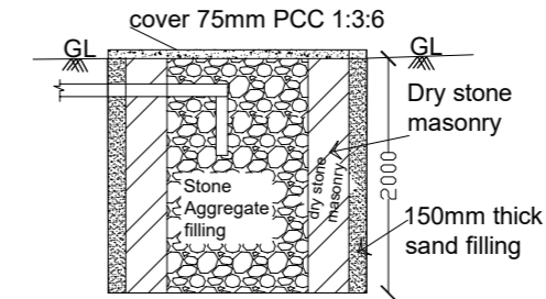
SECTION SOAK PIT
