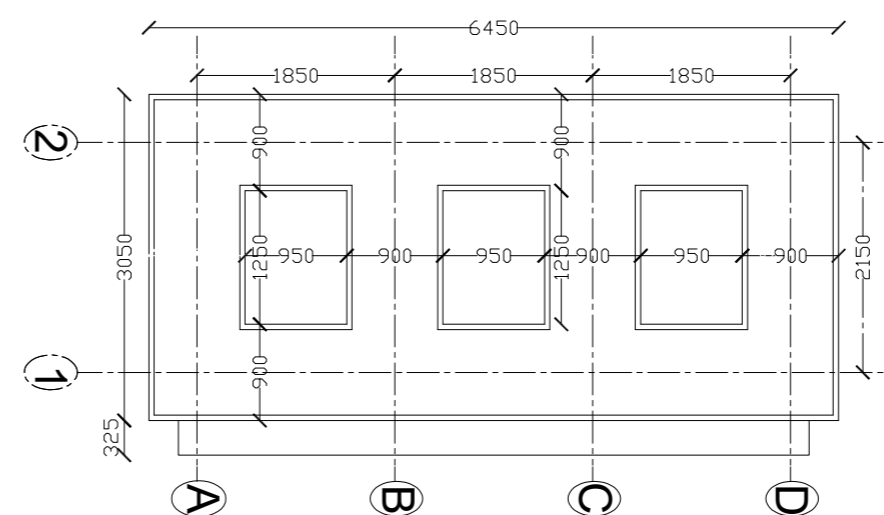
Footing Trench Excavation Plan
