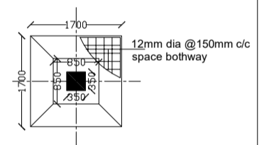
Footing plan Type F1, 1.7mX1.7m
