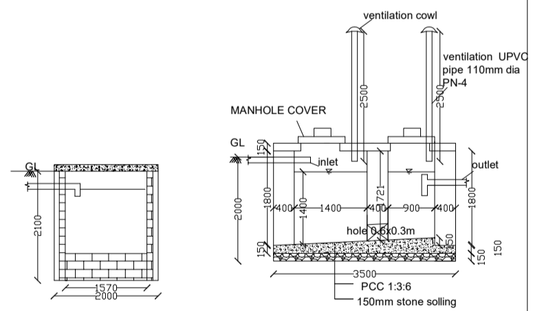
SECTION SOCKPIT
