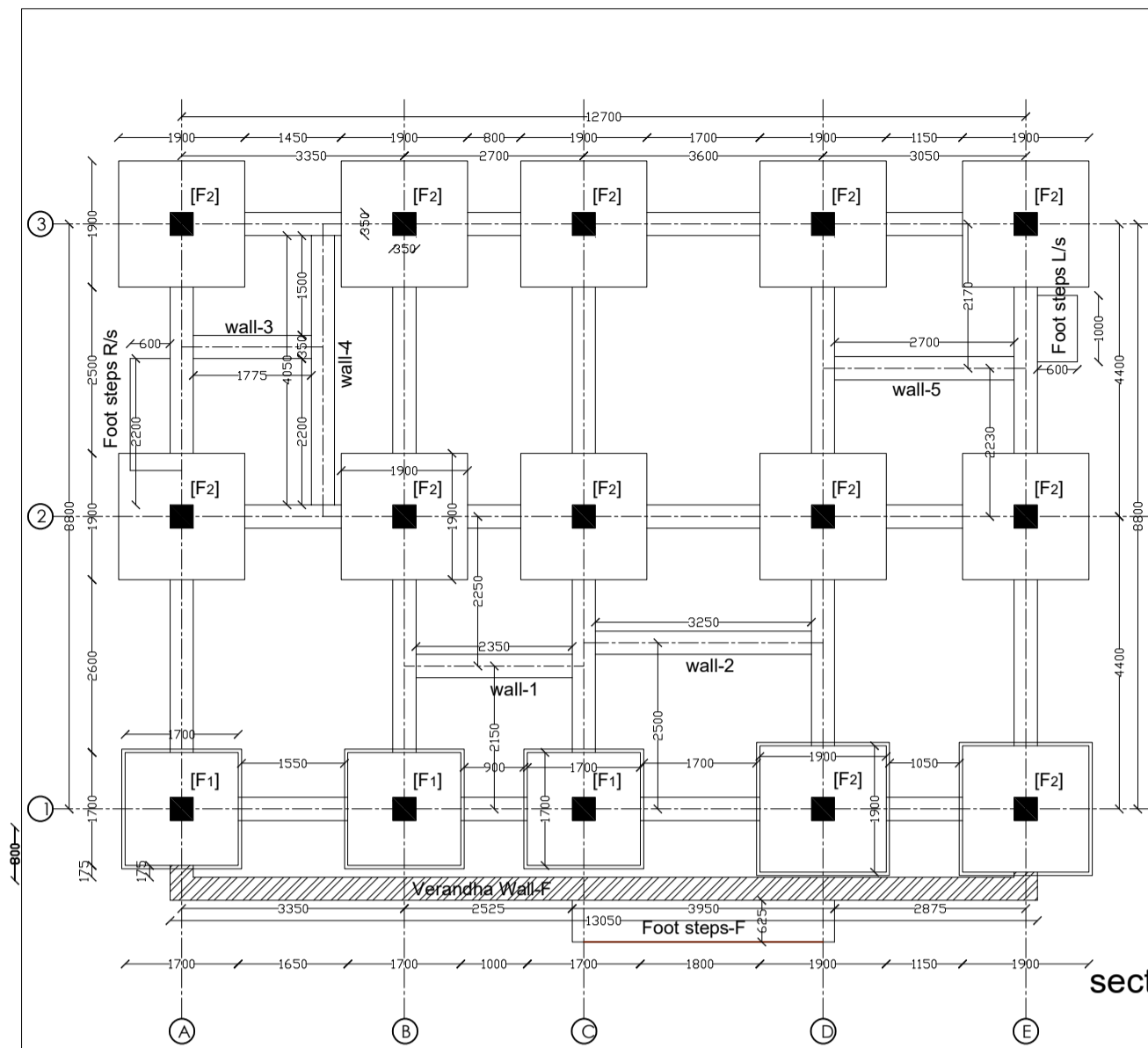
TRANCH EXCAVATION PLAN
