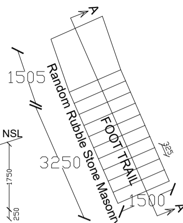
Foot trail Steps Plan
