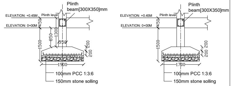
Footing section F2, Type 1.9mX1.9m
