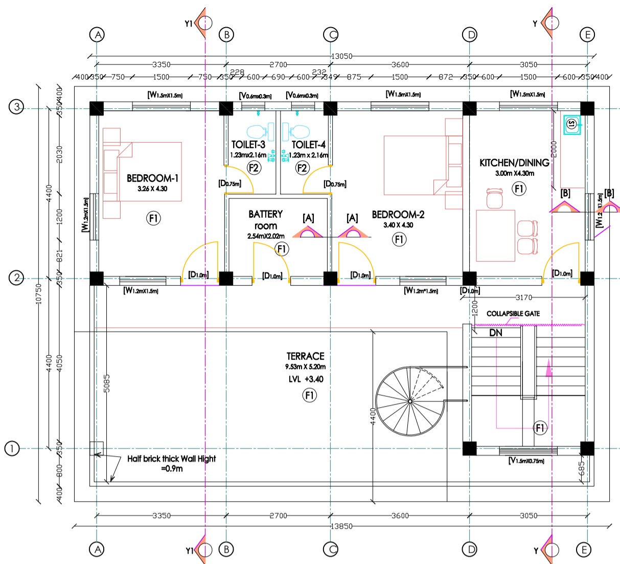
FIRST FLOOR PLAN AREA: 75.30 SQ. M
