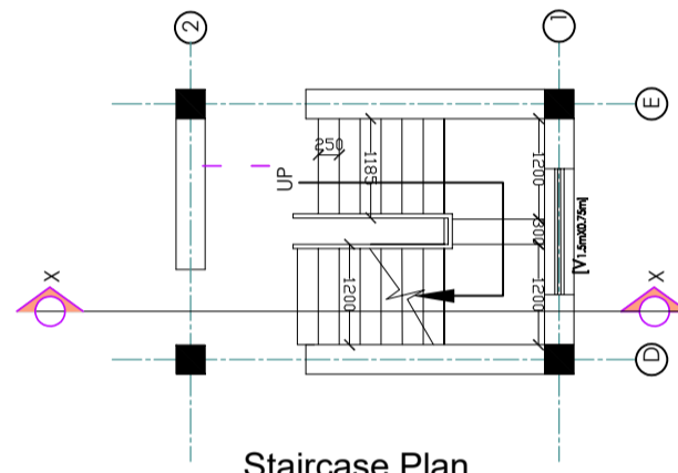
Staircase Plan
