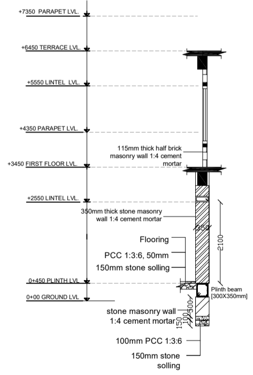
SECTION AT B-B
