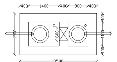
PLAN septic tank 3.5mx2.1m [20users for 2 years]
