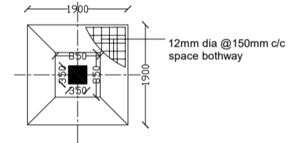
Footing plan Type F2, 1.9mX1.9m
