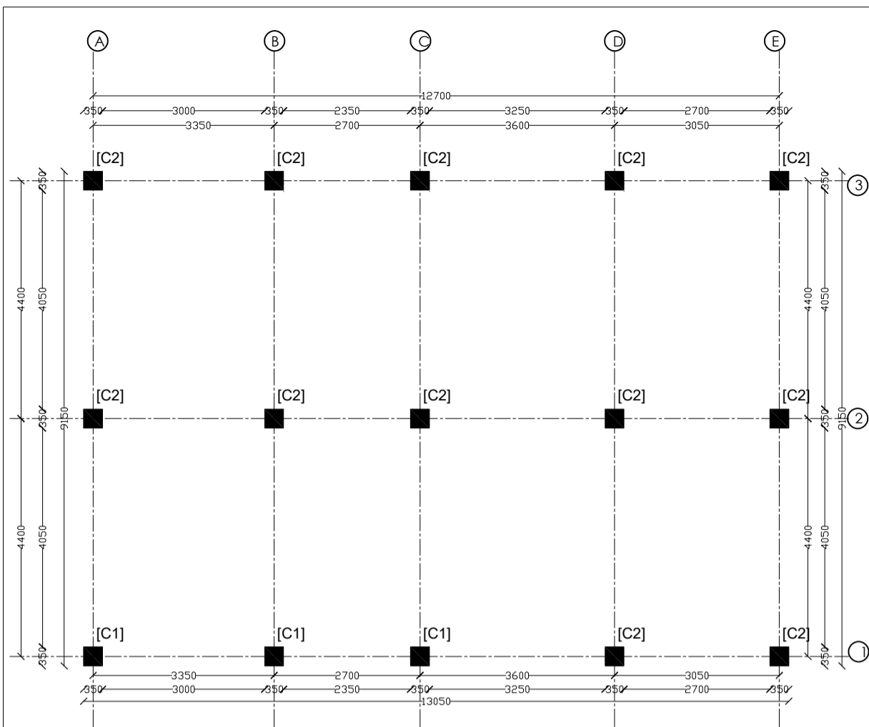
COLUMN PLAN [Size 350mmX350mm]
