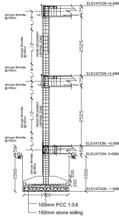
FOOTING & COLUMN F2 Type
