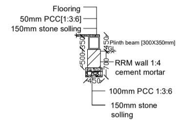
section grid 1,2,3, A,B,C,D,E and wall 1,2,3,4&5
