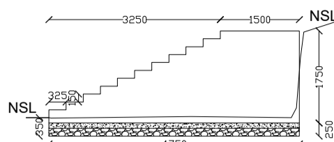
Foot trail Steps section
