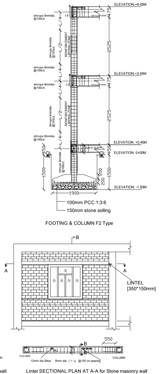
Lintel SECTIONAL PLAN AT A-A for Stone masonry wall
