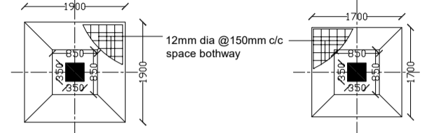
Footing plan Type F2, 1.9mX1.9m
