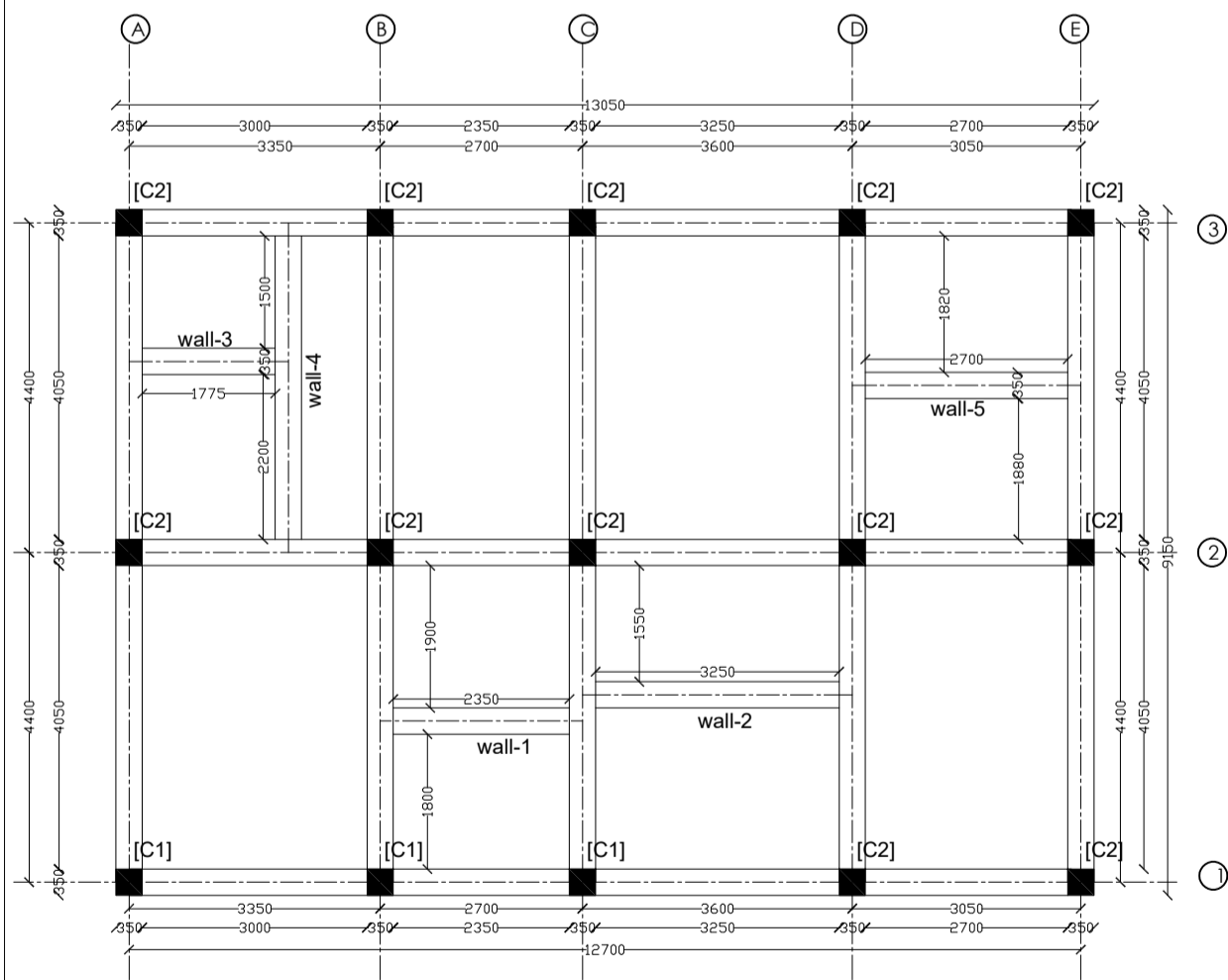
Plinth Tie Beam Layout PLAN [Size 300mmX350mm]
