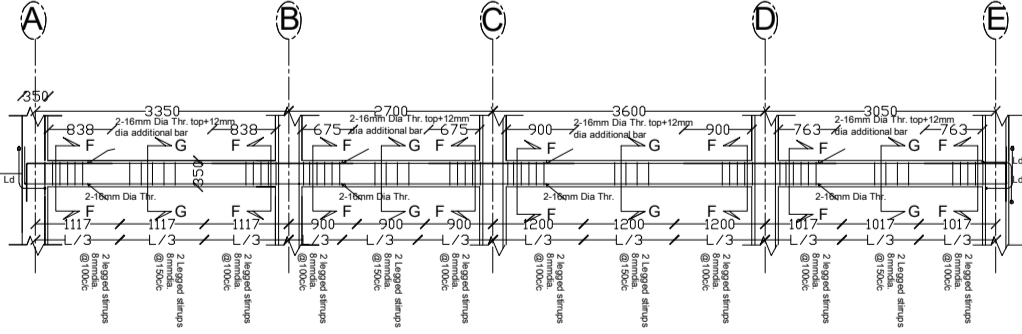
FIRST FLOOR BEAM L-Section along 2 & 3
