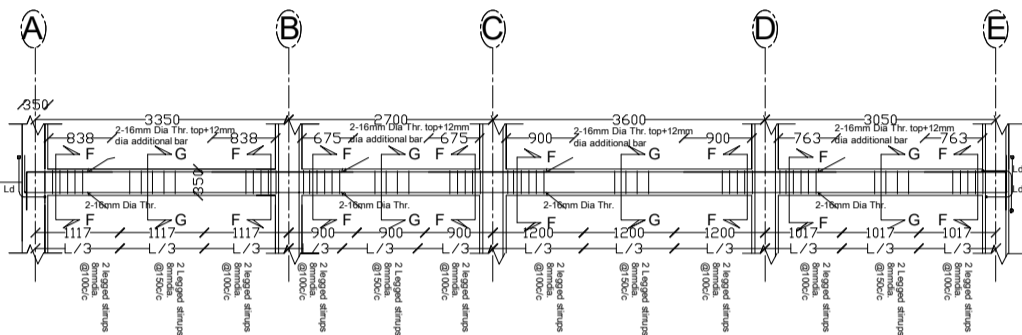
FIRST FLOOR BEAM L-Section along 1-1
