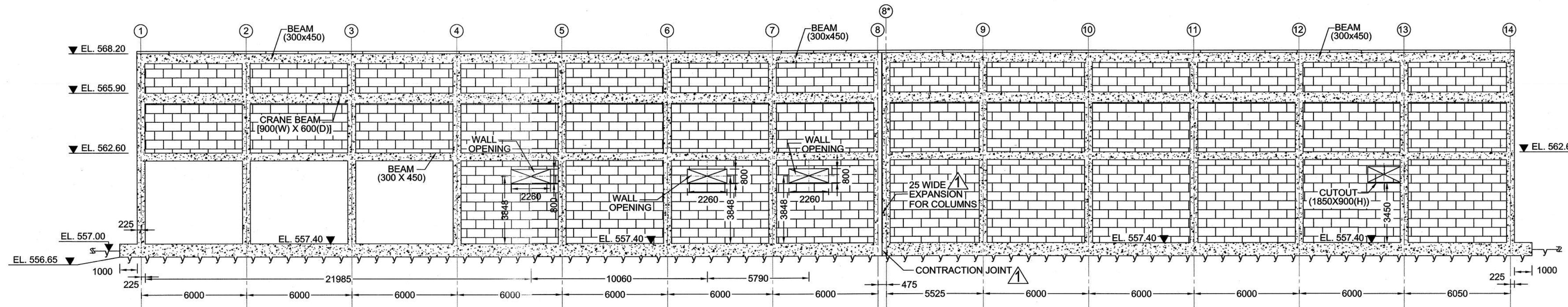
SECTION B-B
