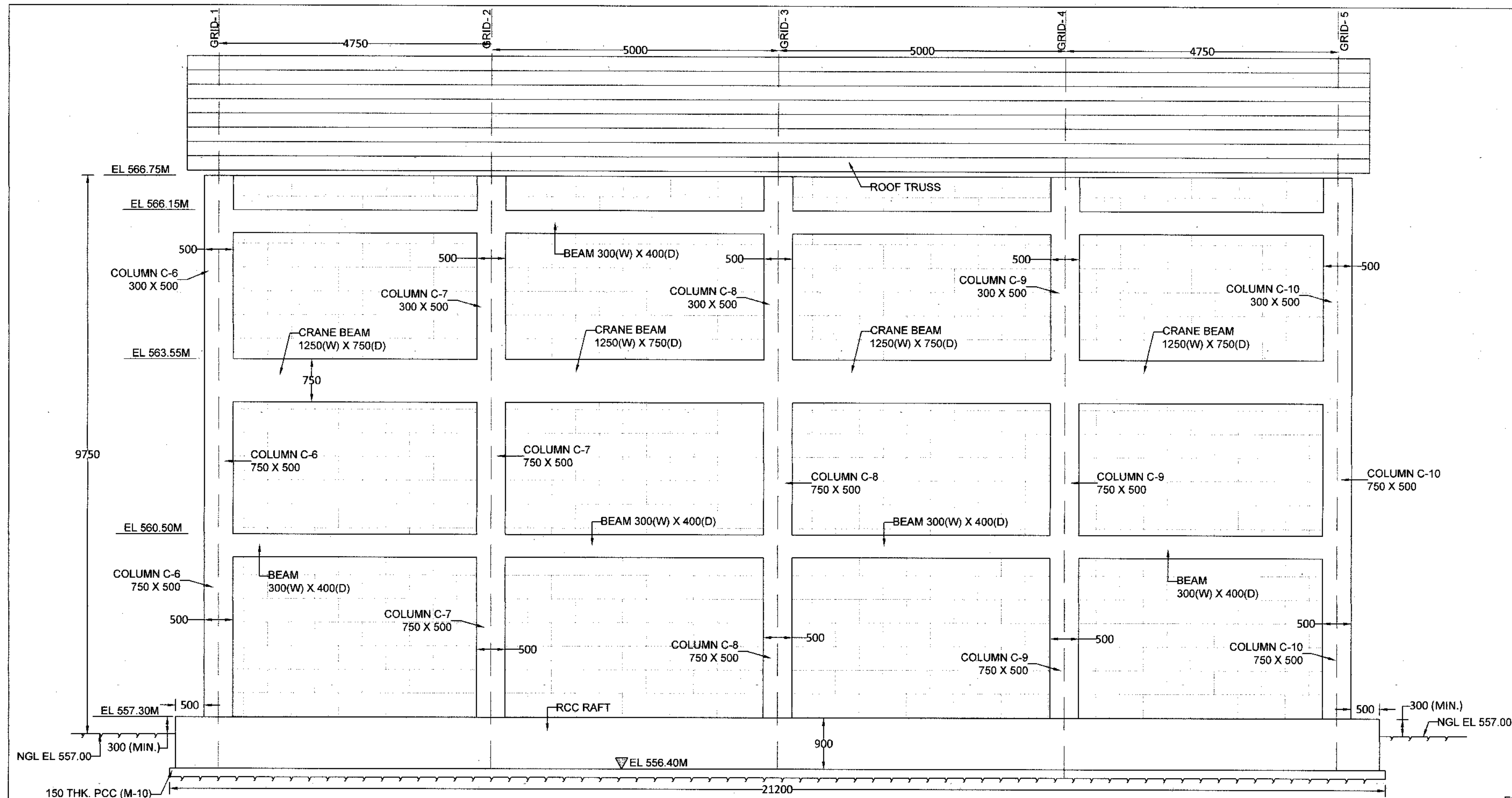
VIEW "3"
