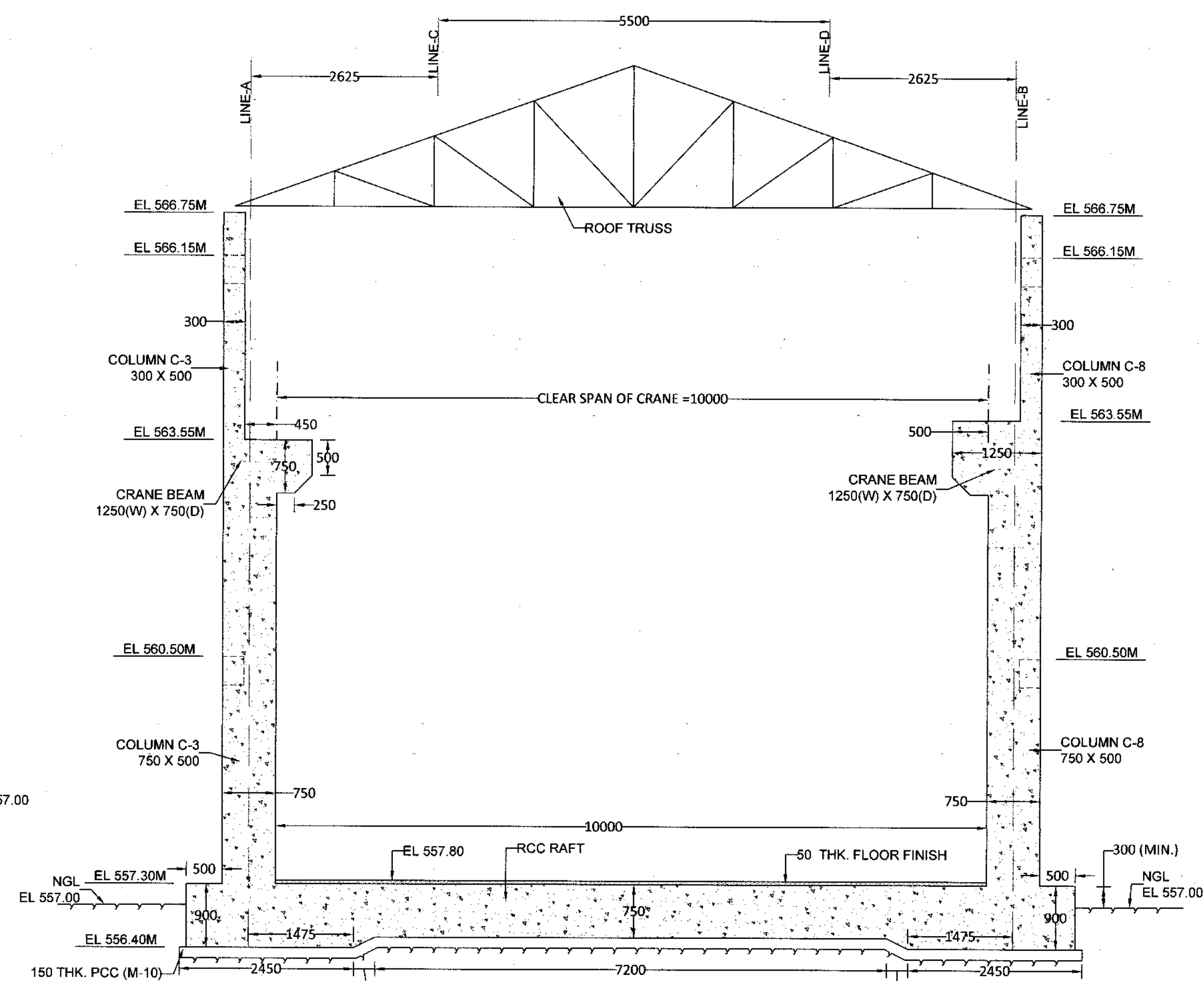
SECTION R-R
