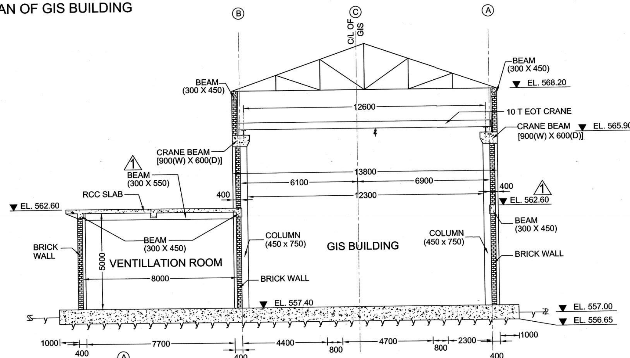
△ SECTION 12-12
