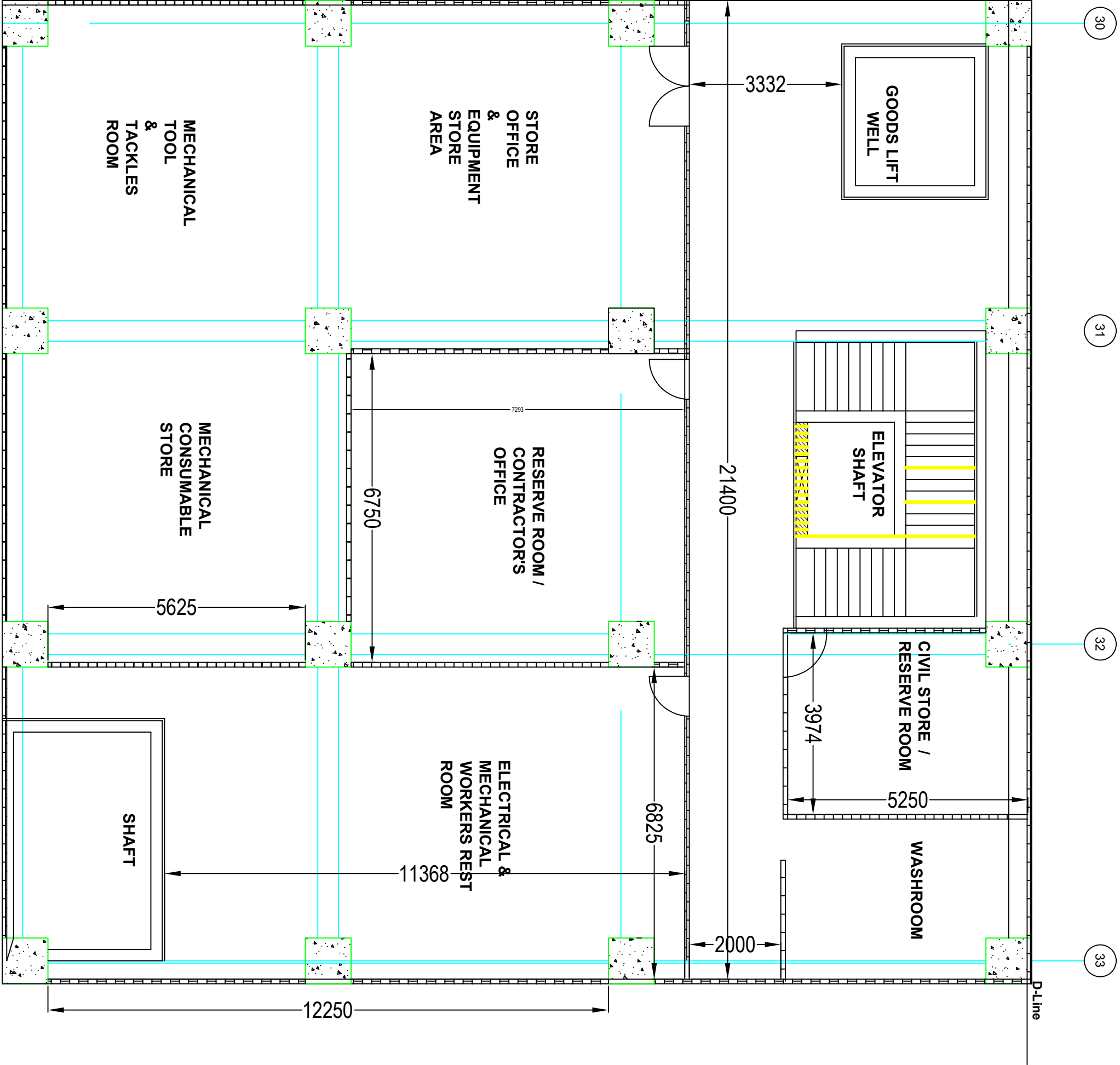
FLOOR PLAN FOR EL.523 (MIV Floor)
