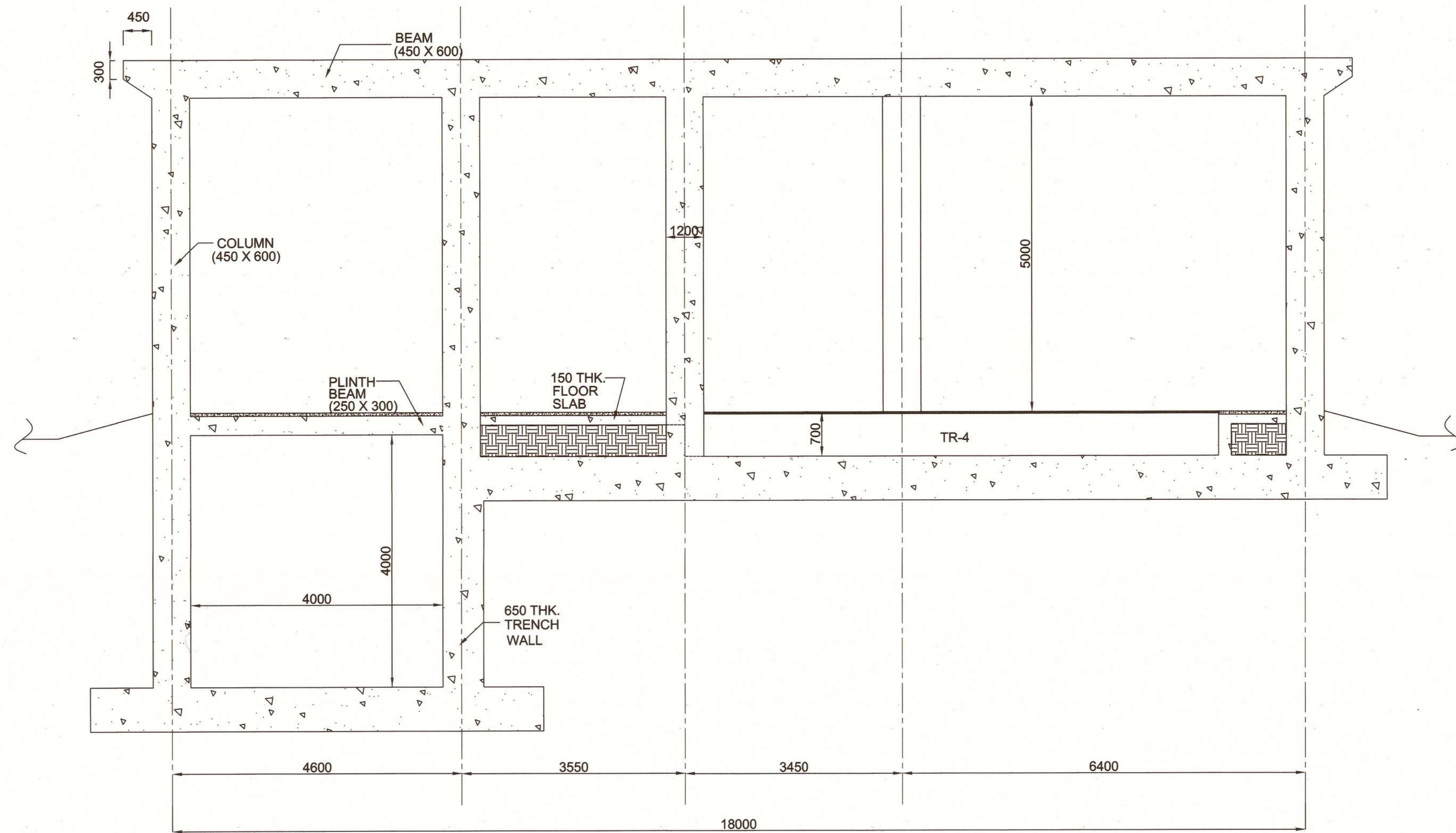
SECTION B-B
