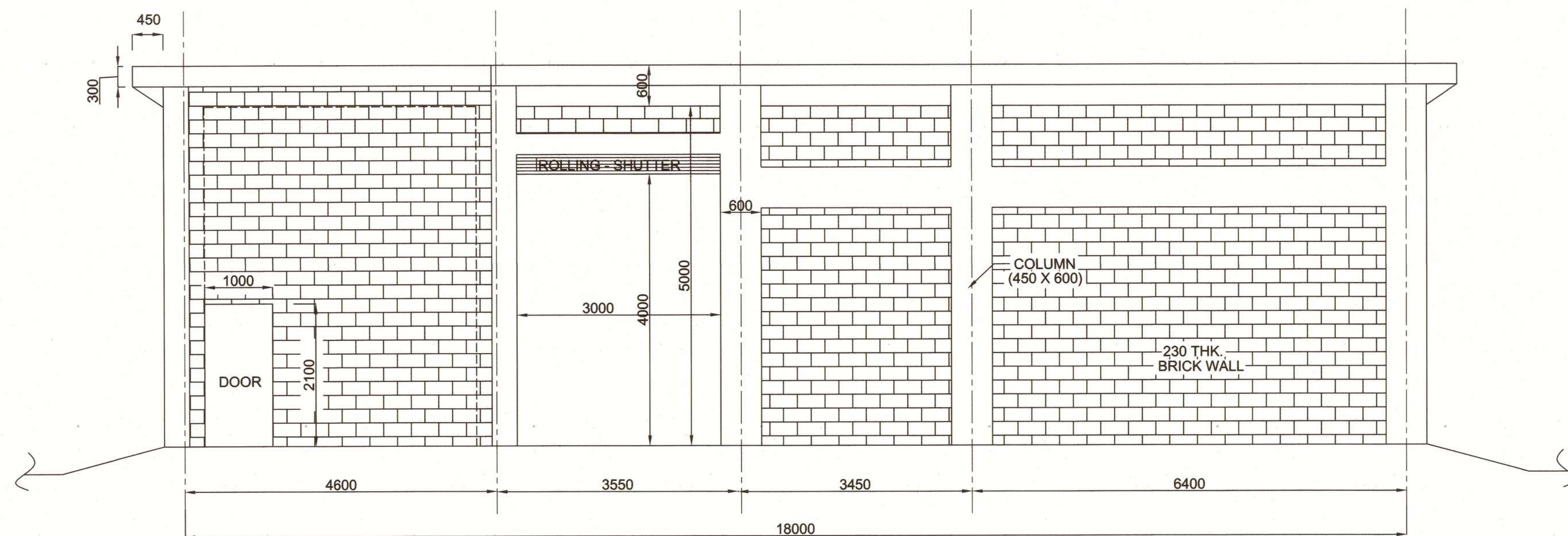
VIEW-B
