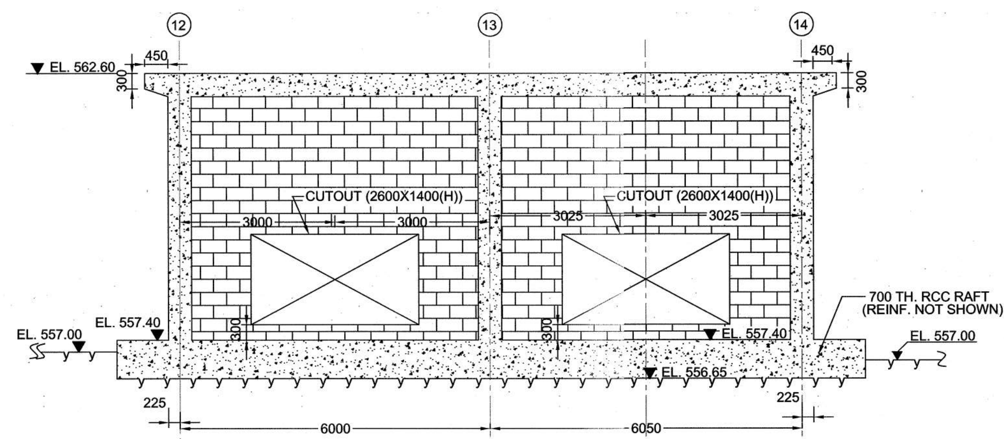
SECTION G-G
