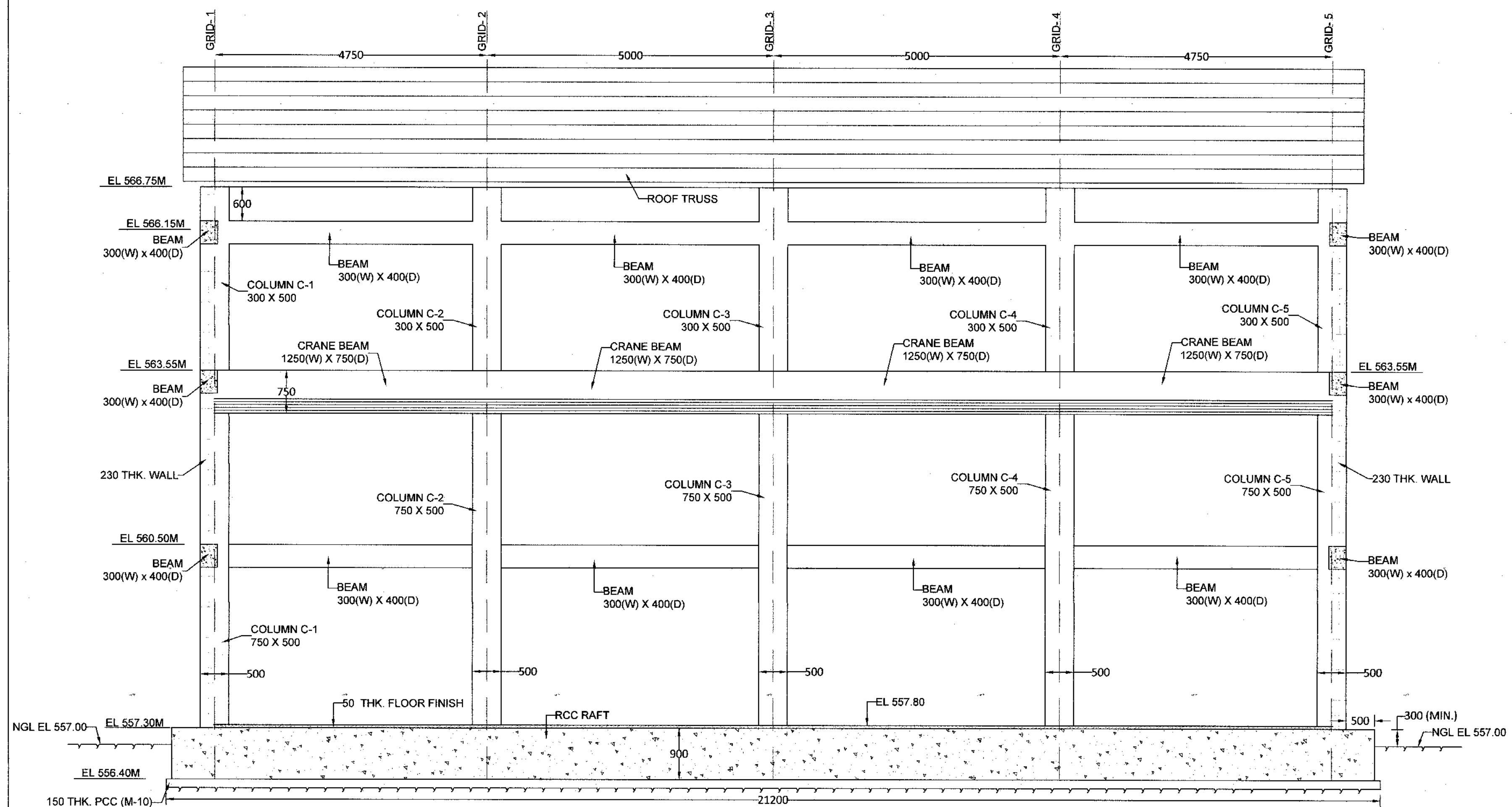
SECTION P-P
