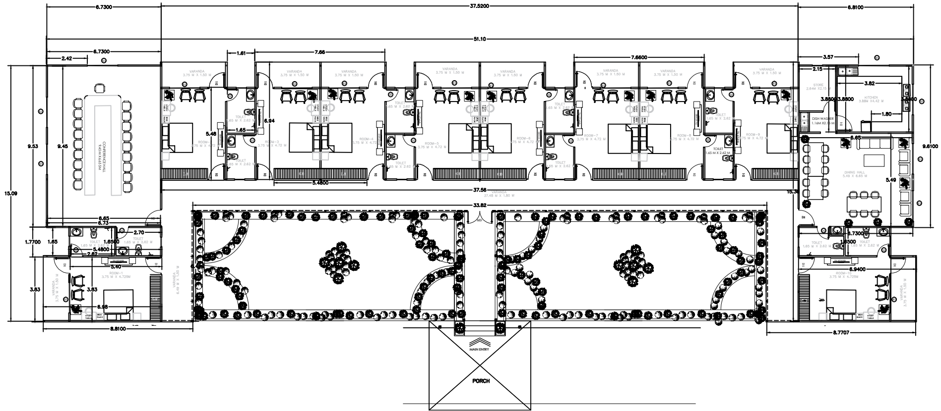
TEMPORARY GUEST HOUSE PLAN AT SURGE SHAFT
