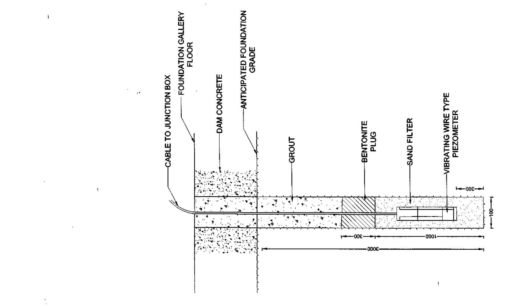
TYPICAL BOREHOLE INSTALLATION OF VIBRATING WIRE TYPE PIEZOMETER (NOT TO SCALE)
