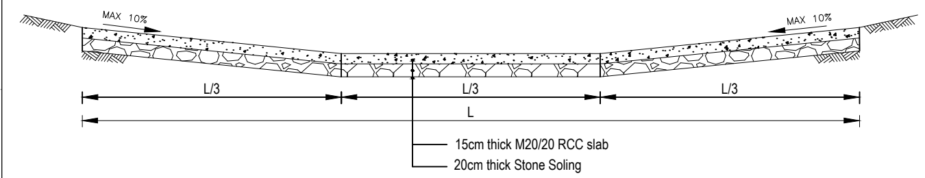
Section at B-B Scale 1:100
