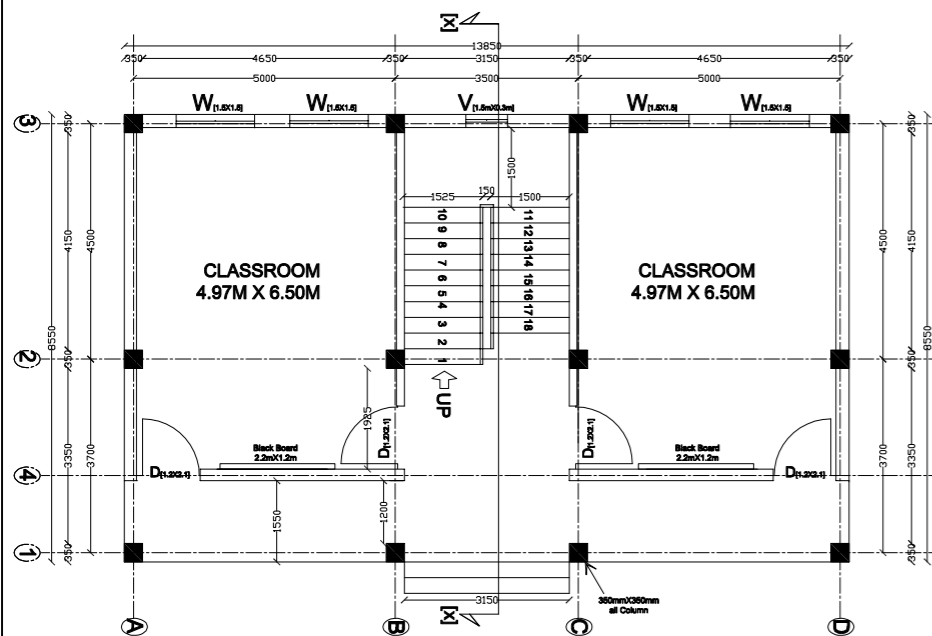
GROUND FLOOR PLAN PLINTH AREA : 118.42sq.m
