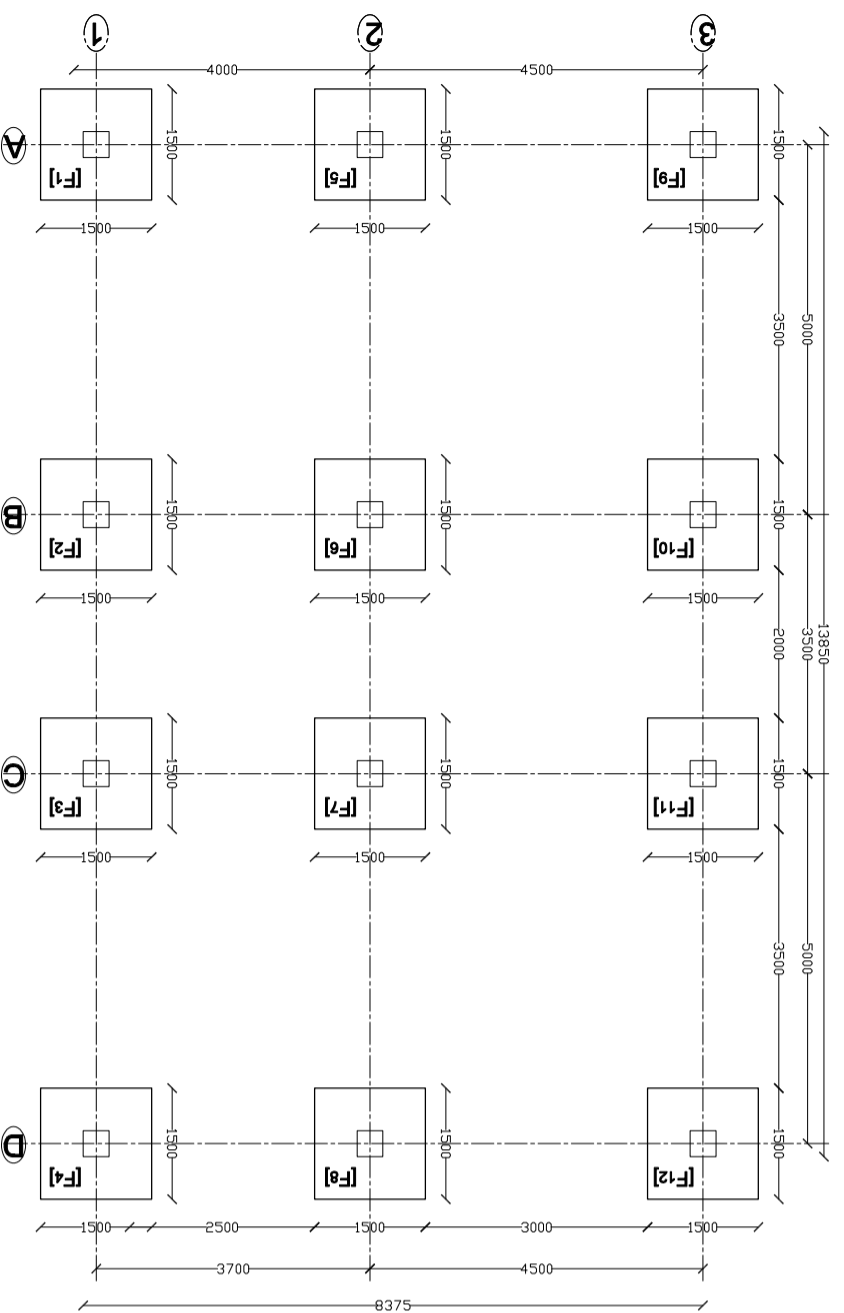
FOOTING PLAN
