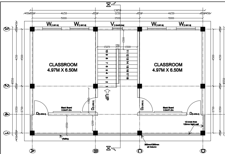
First FLOOR PLAN PLINTH AREA : 118.42sq.m
