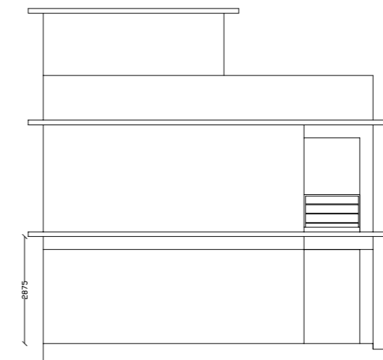
NORTH ELEVATION
