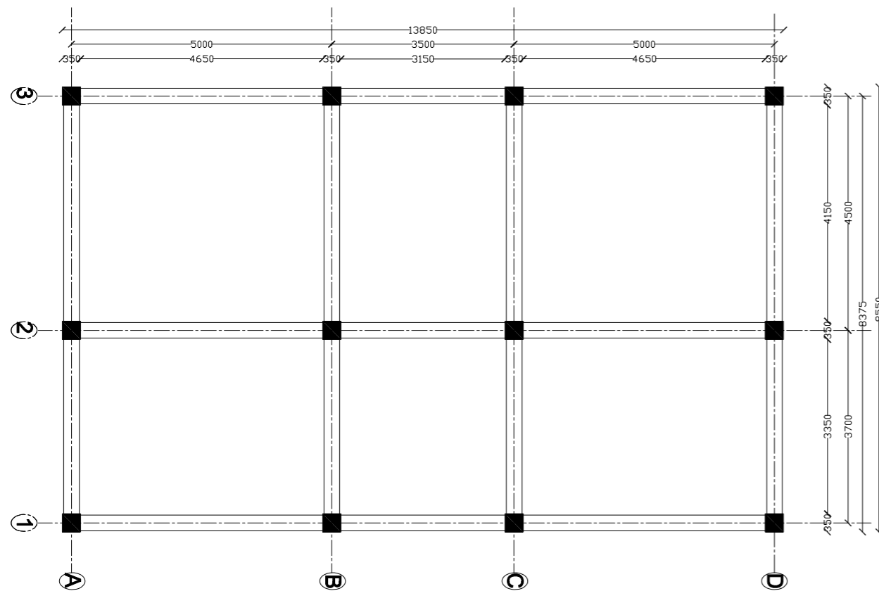
FLOOR BEAM LAYOUT PLAN [clear-section 350*300mm]
