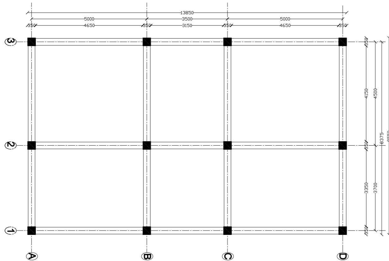
PLINTH BEAM LAYOUT PLAN [350*300mm]
