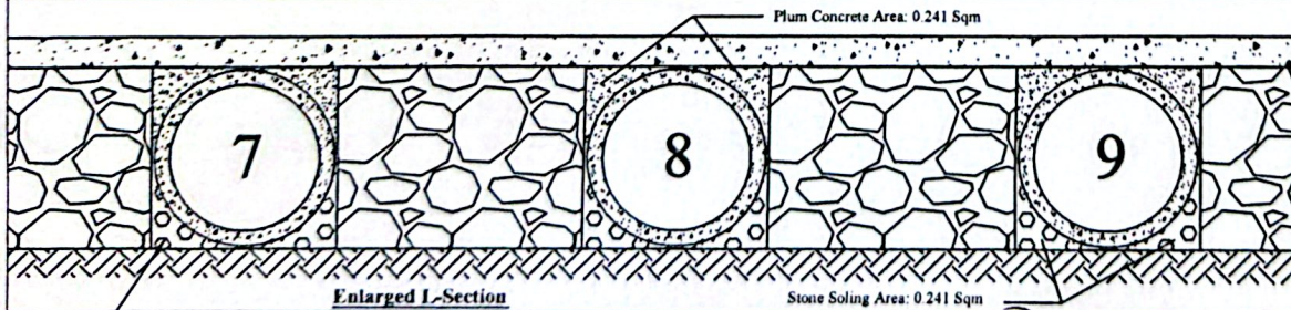
Enlarged I-Section
